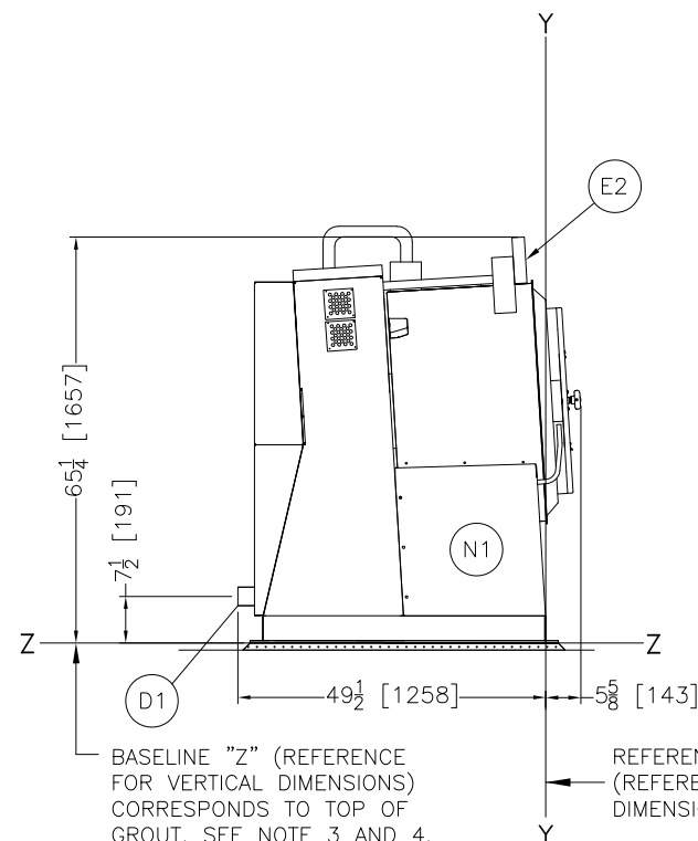
LEFT VIEW
