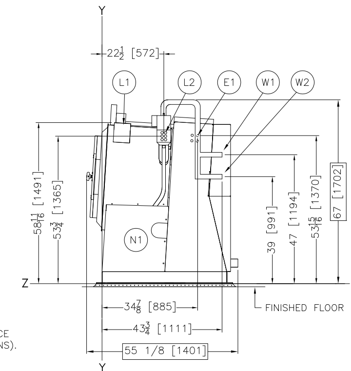
RIGHT VIEW
