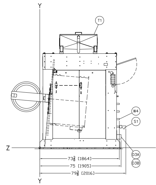
RIGHT VIEW
