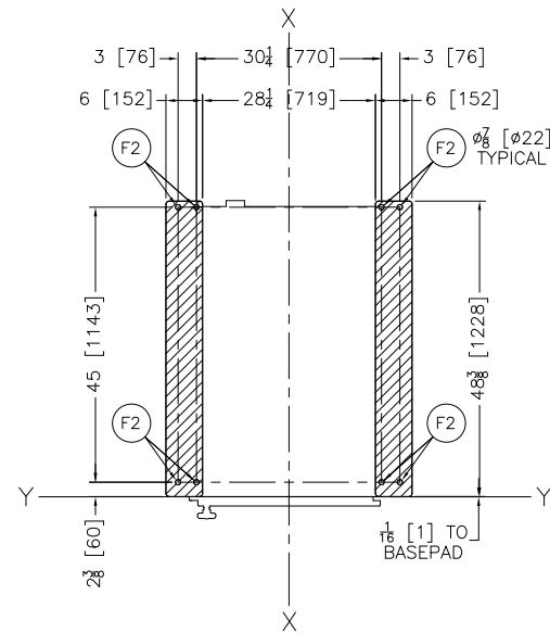
FOUNDATION PLAN
