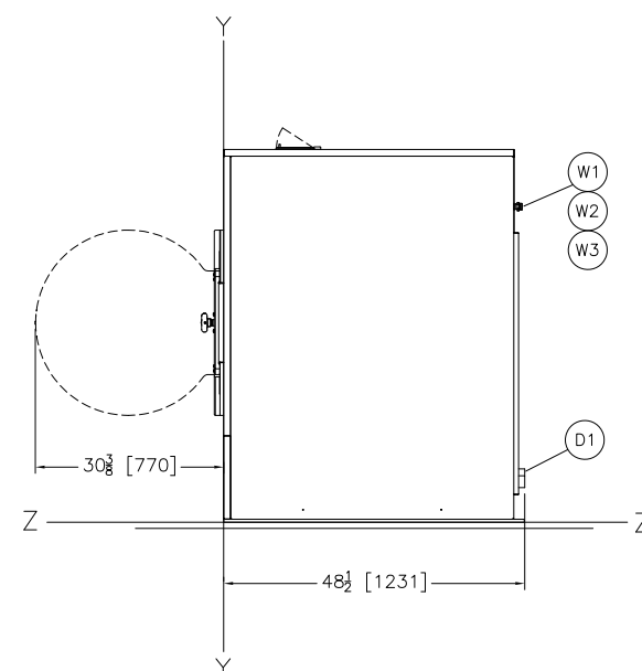
RIGHT VIEW
