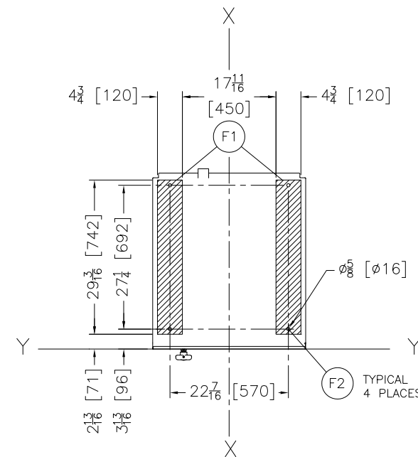
FOUNDATION PLAN
