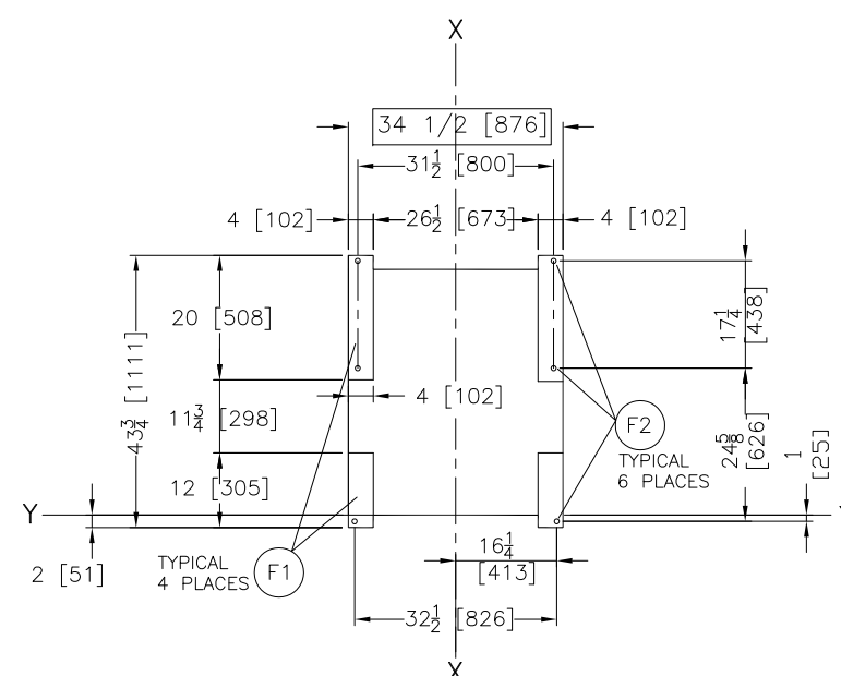
FOUNDATION VIEW
