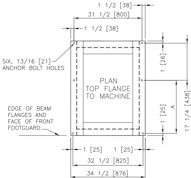
DETAIL B
