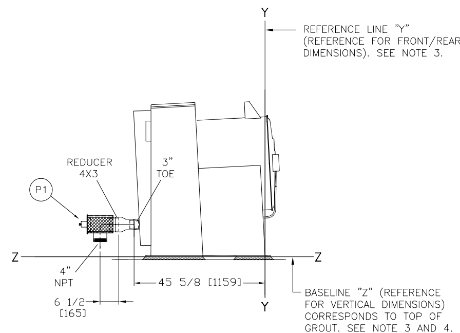
LEFT VIEW
