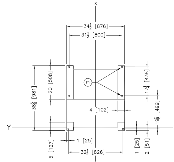
FOUNDATION VIEW
