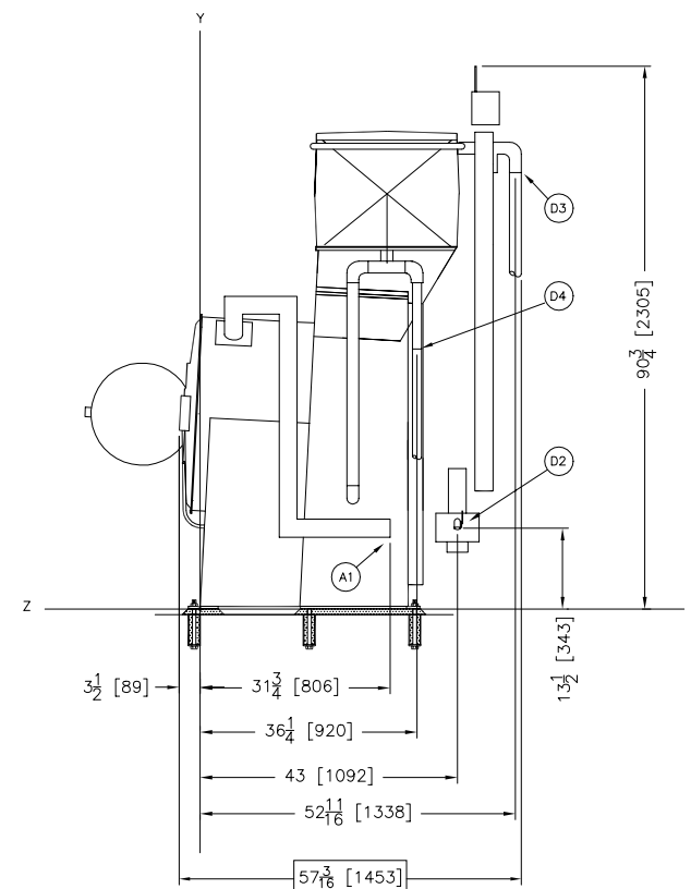
RIGHT VIEW
