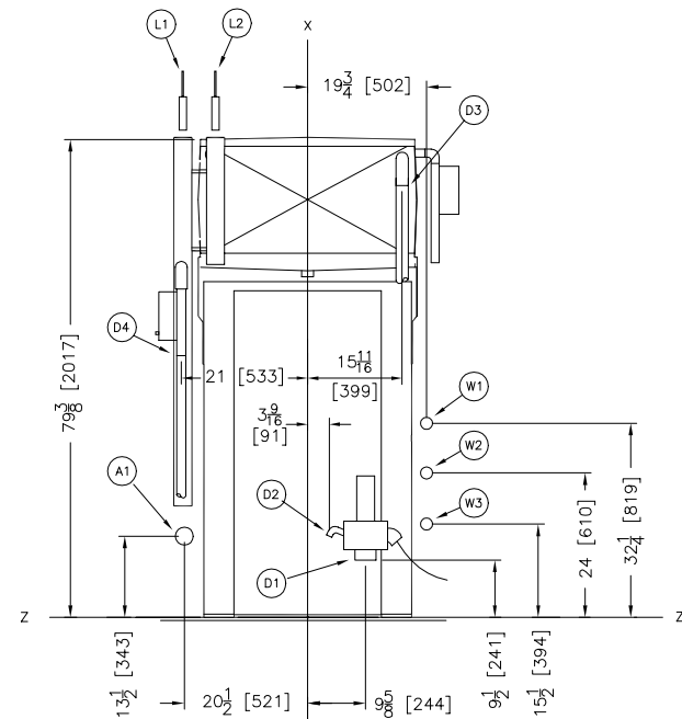
REAR VIEW
