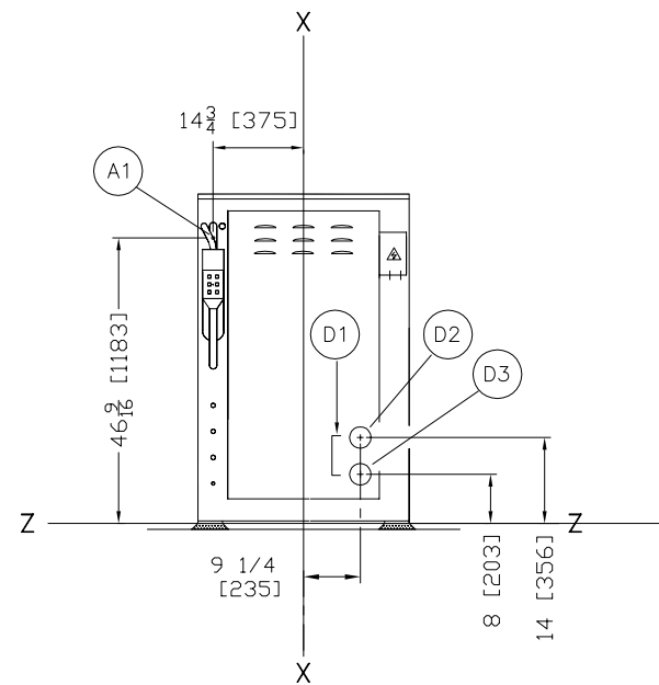
REAR VIEW
