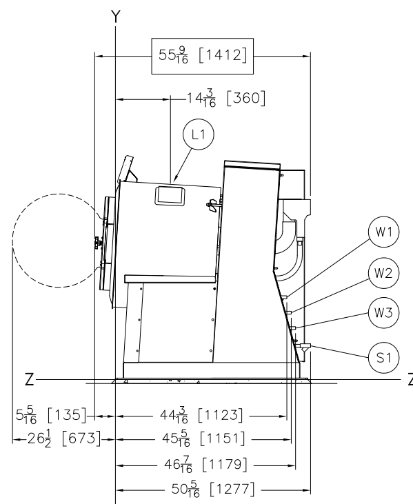
RIGHT VIEW
