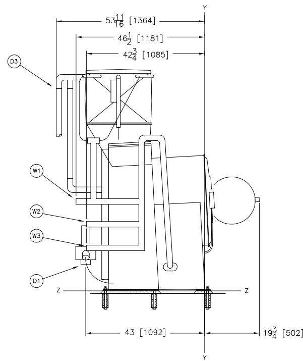
LEFT VIEW
