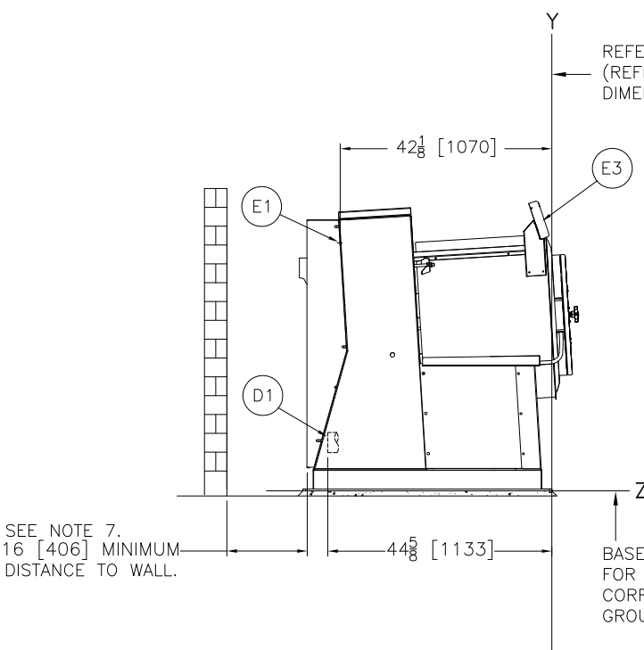
LEFT VIEW
