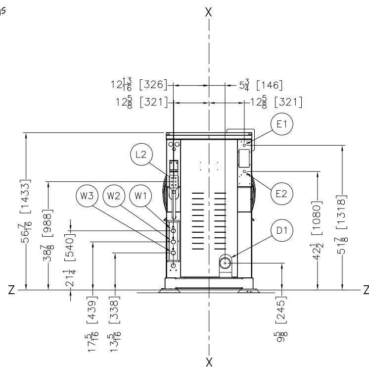
REAR VIEW
