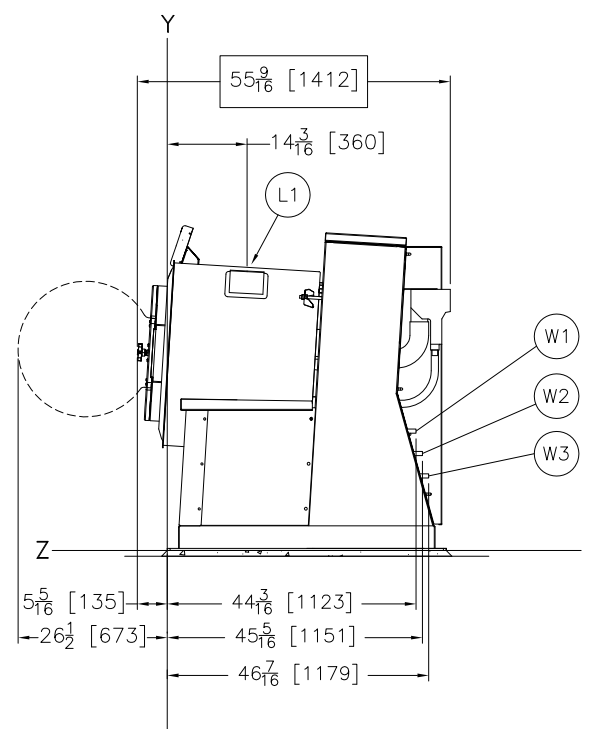
RIGHT VIEW
