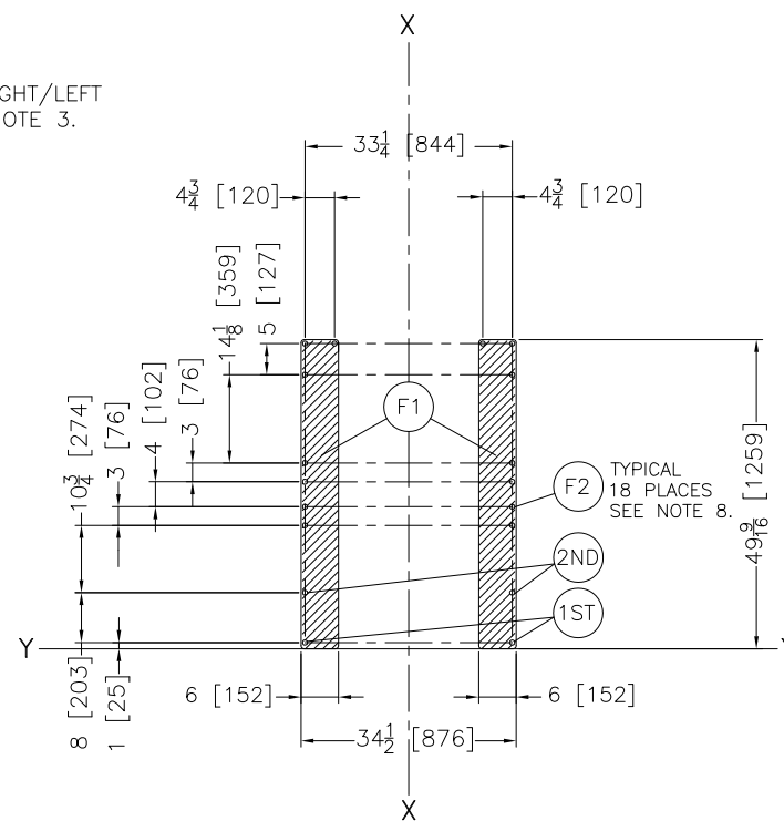
FOUNDATION VIEW
