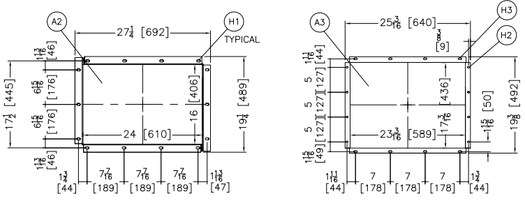
BLOWER INTAKE DUCT DETAIL VIEW A-A
