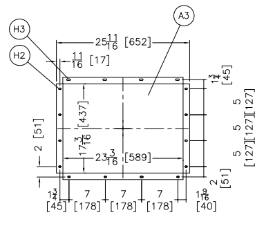
RECIRCULATION BLOWER EXHAUST TO REAR DUCT DETAIL
