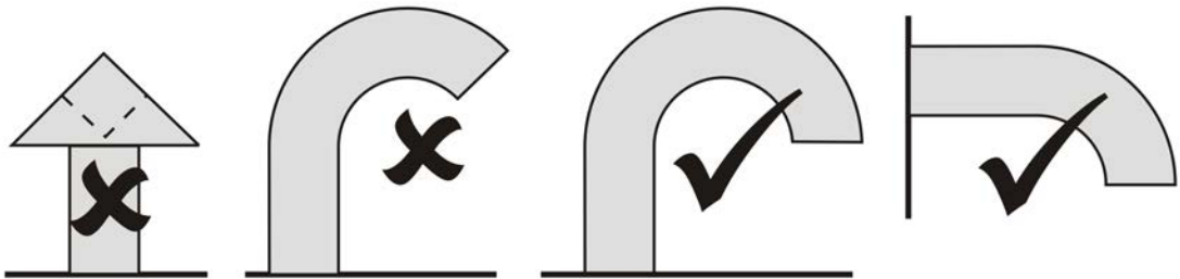
Figure 2. Vent Designs
