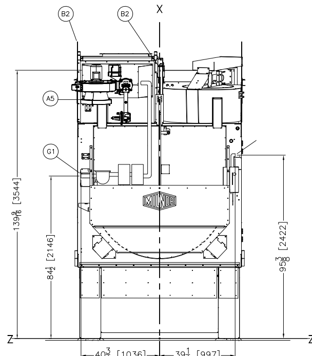
REAR VIEW
