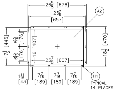
RECIRCULATION DUCT BLOWER INTAKE DETAIL
