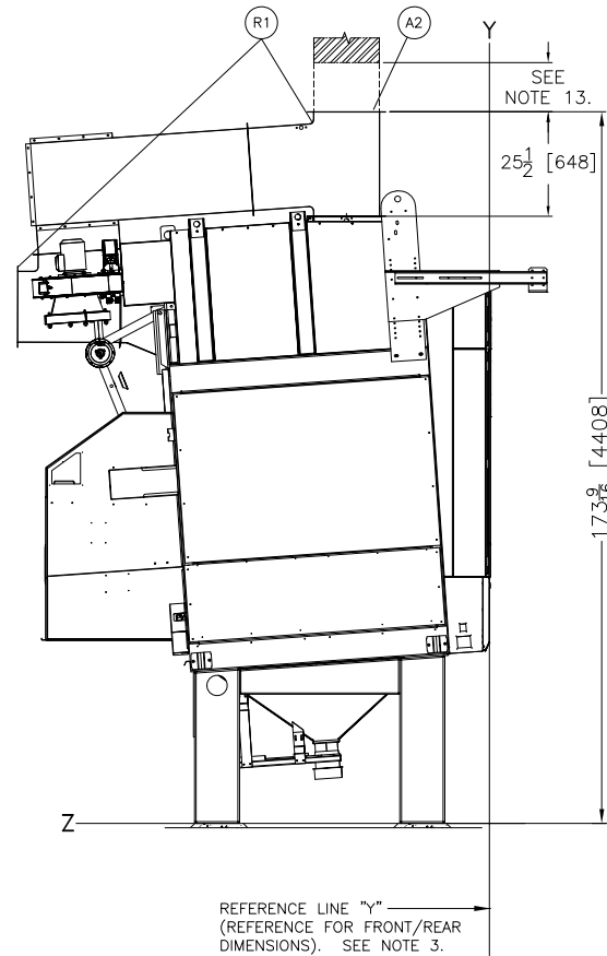
LEFT VIEW
