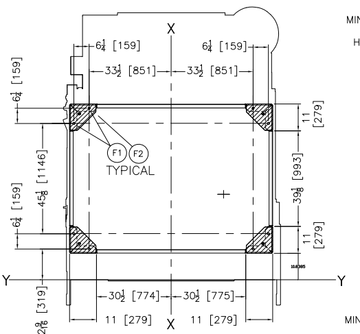
FOUNDATION PLAN
