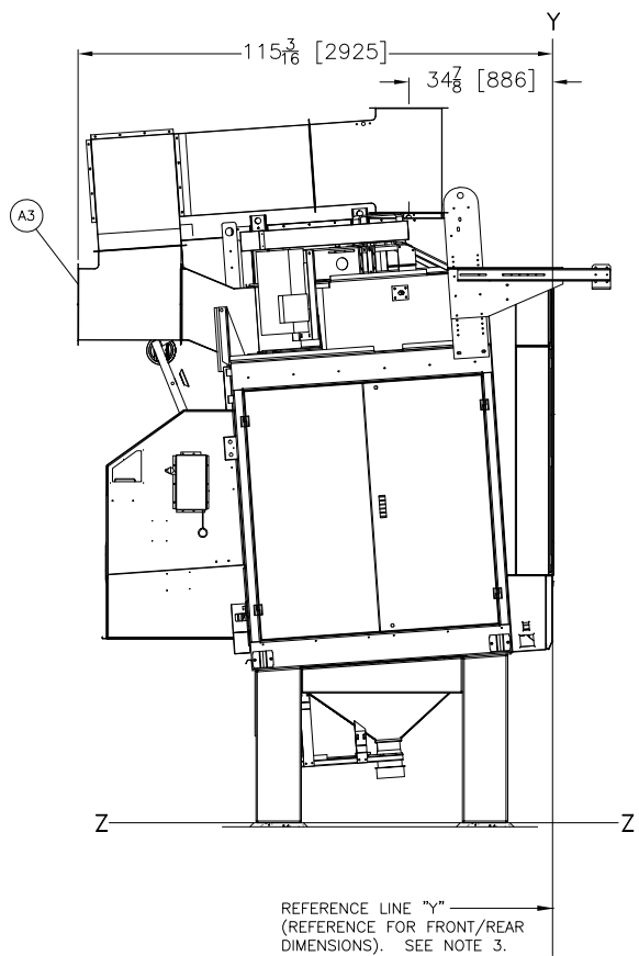
LEFT VIEW
