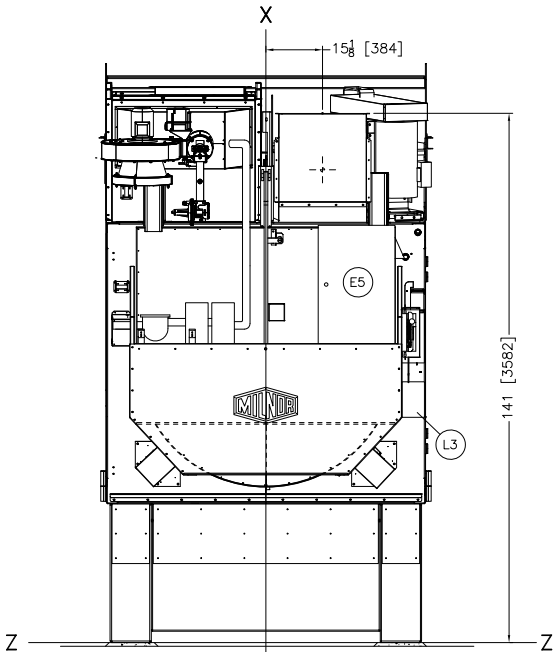
REAR VIEW
