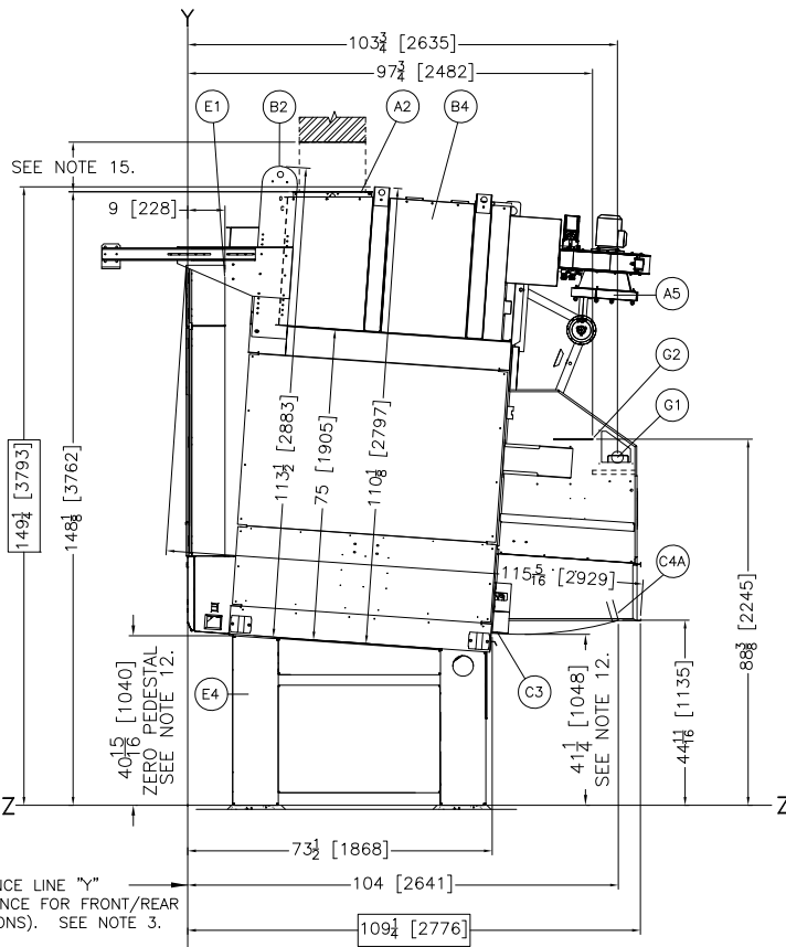
RIGHT VIEW
