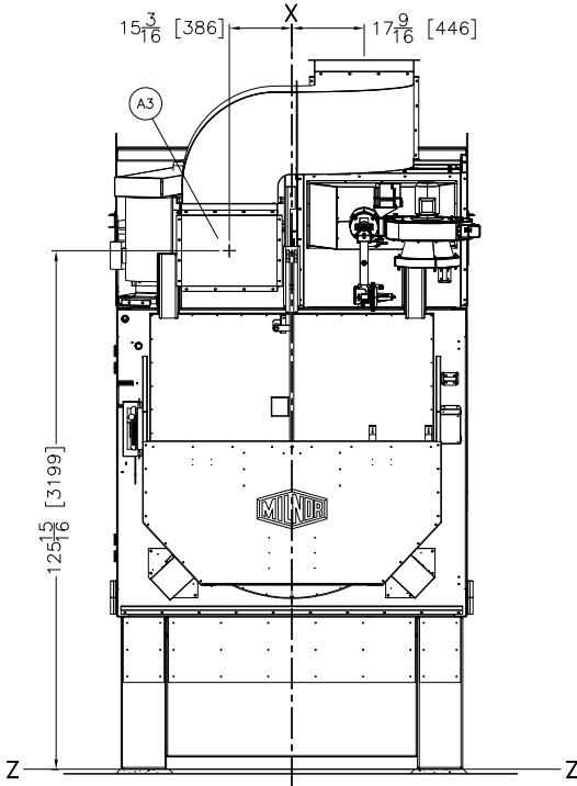
REAR VIEW
