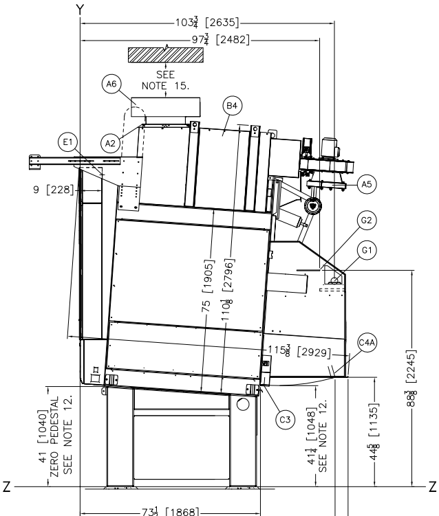
REAR VIEW
