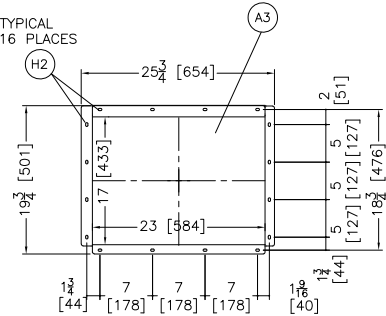
RECIRCULATION DUCT UP DETAIL
