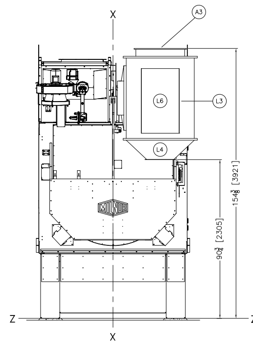
REAR VIEW LINT OUTLET TO BAG COLLECTOR
