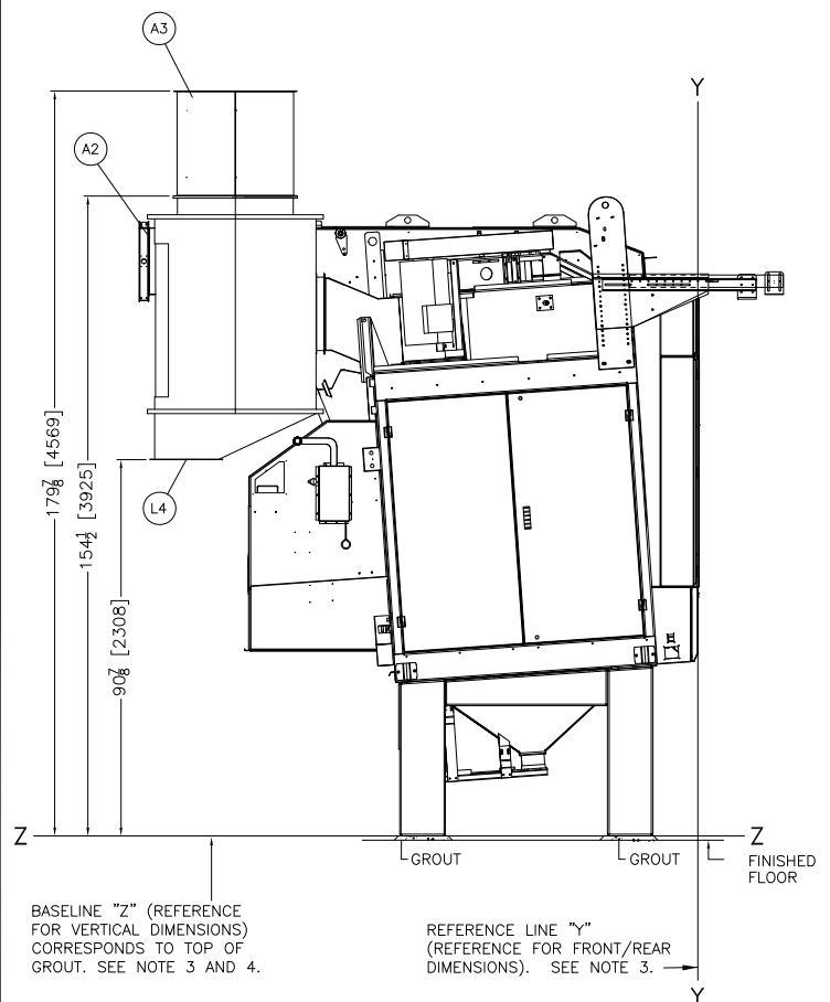
LEFT VIEW LINT OUTLET TO BAG COLLECTOR
