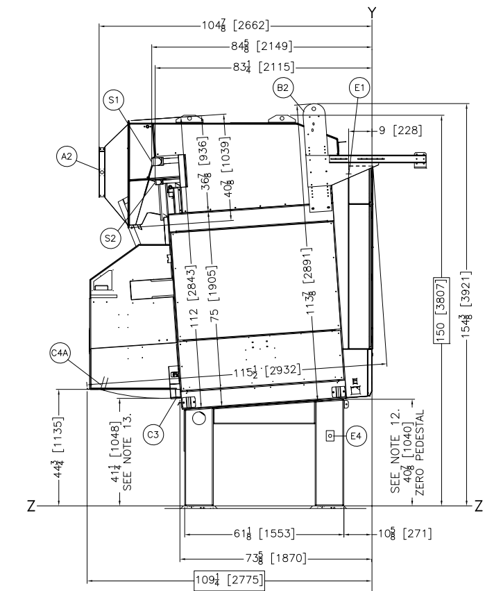
LEFT VIEW
