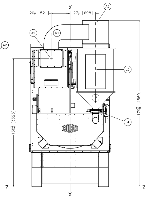
REAR VIEW LINT OUTLET TO VACUUM COLLECTOR
