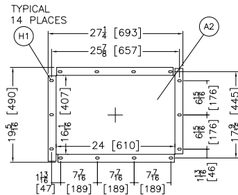
RECIRCULATION BLOWER INTAKE DUCT DETAIL
