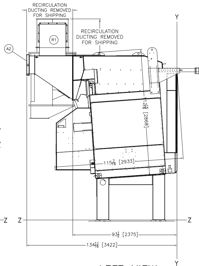
LEFT VIEW LINT OUTLET TO BAG COLLECTOR
