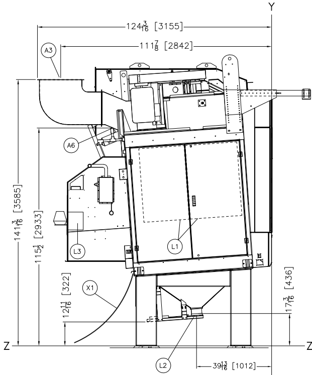
LEFT VIEW
