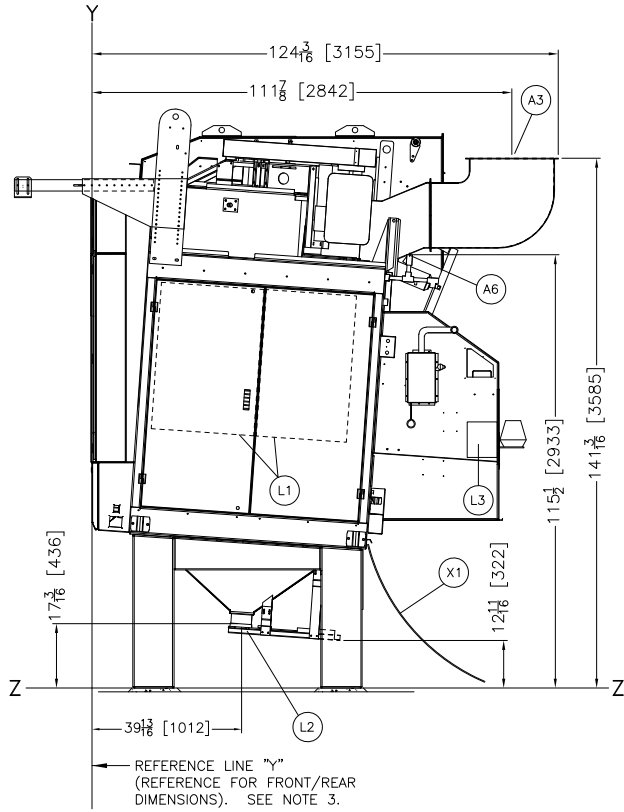
RIGHT VIEW
