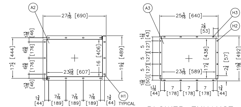
BLOWER EXHAUST DUCT TO REAR DETAIL SEE NOTE 13.
