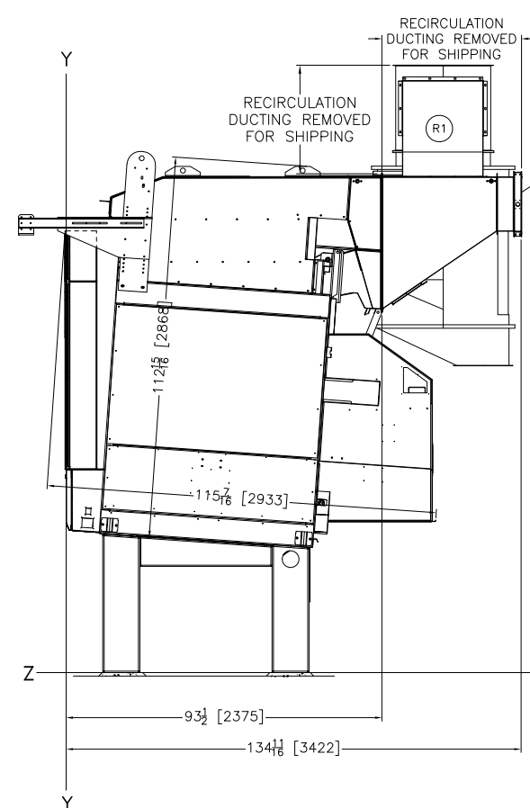
RIGHT VIEW
