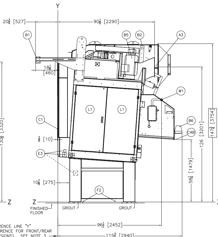
RIGHT VIEW
