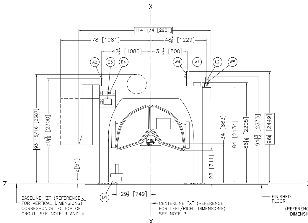
FRONT VIEW
