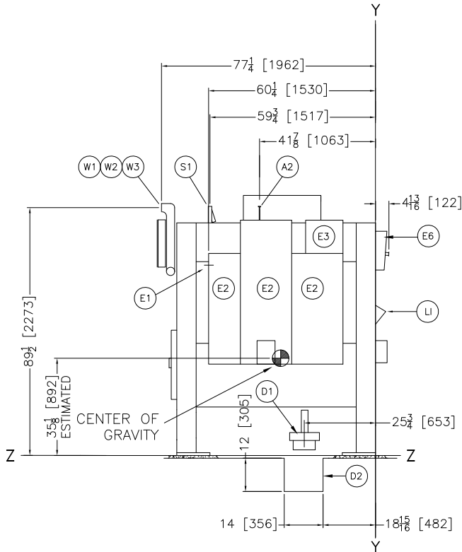
LEFT VIEW
