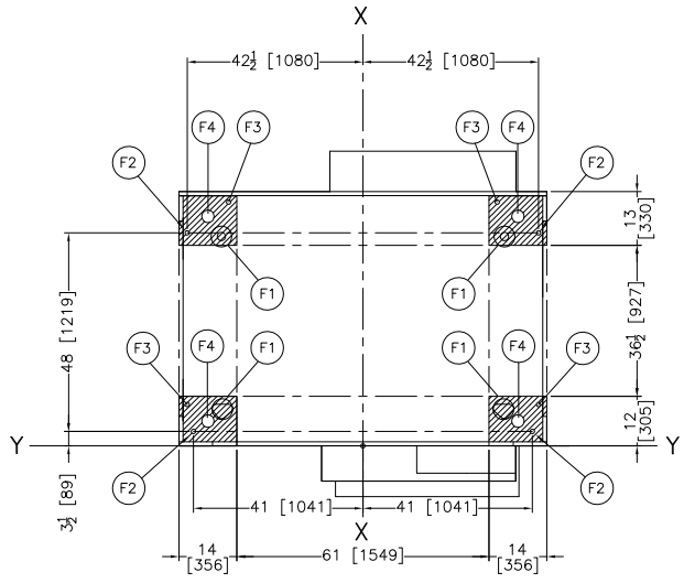
FOUNDATION PLAN
