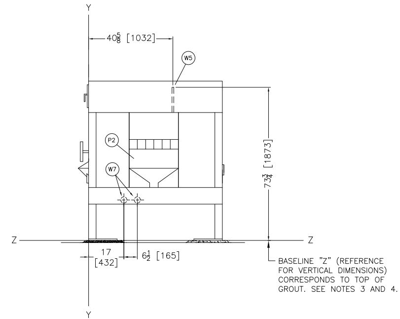
RIGHT VIEW
