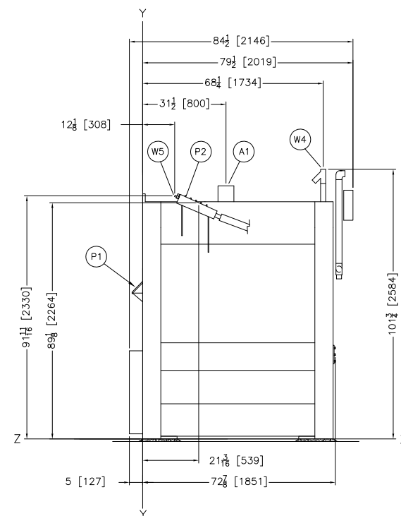
RIGHT VIEW
