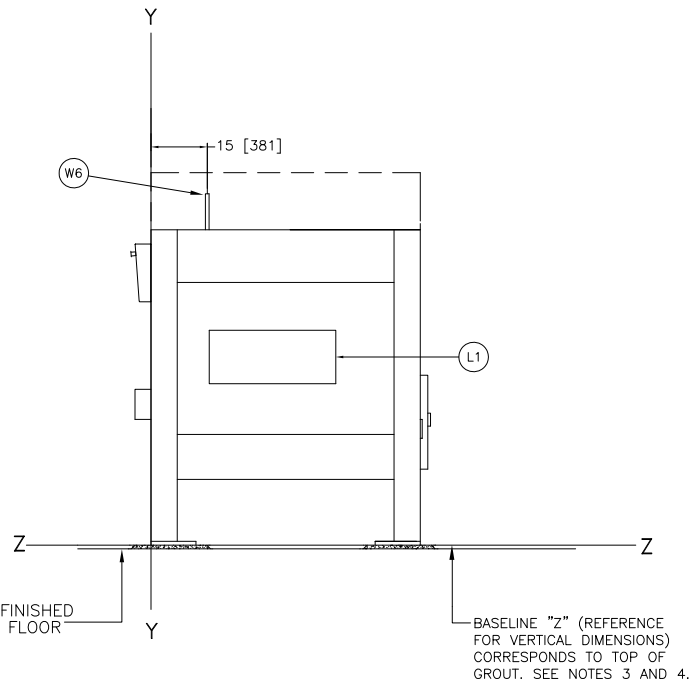
RIGHT VIEW
