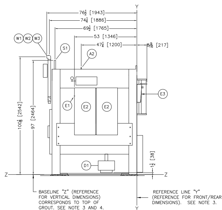
LEFT VIEW
