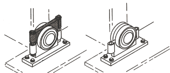
FIGURE 8 (MSIN0203AE) Tilt Wheel Clamps (BTN and BTL models only)
