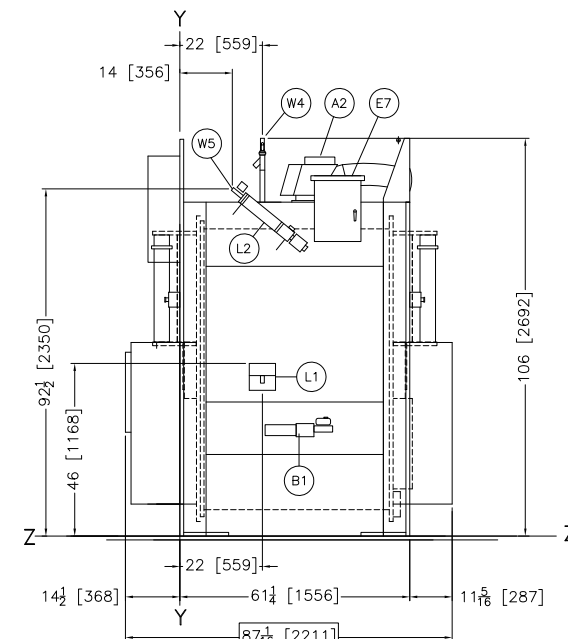
RIGHT VIEW
