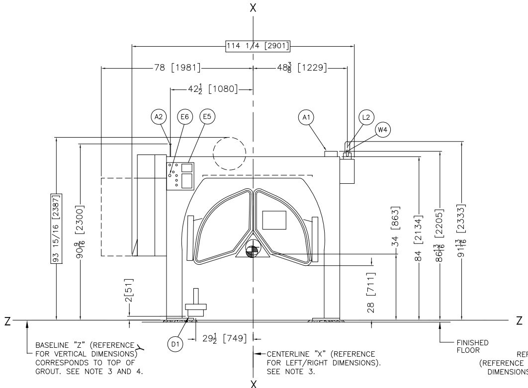
FRONT VIEW
