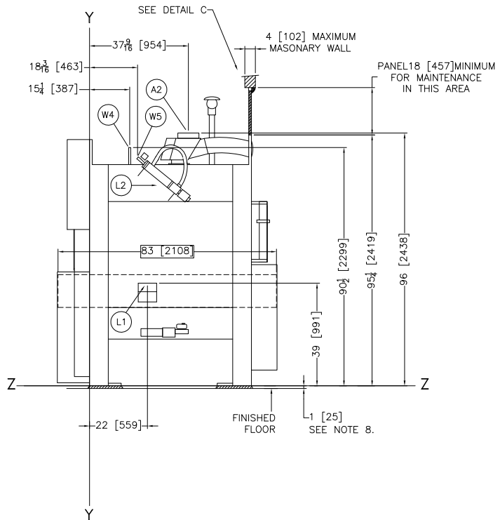
RIGHT VIEW
