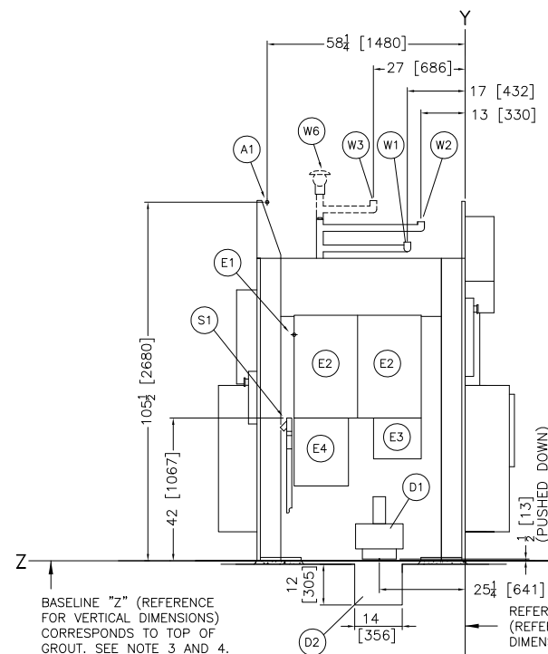
LEFT VIEW
