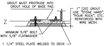
RECOMMENDED DECK MOUNTING DETAIL
