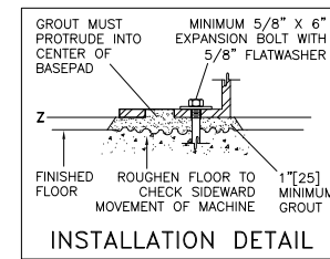
INSTALLATION DETAIL
