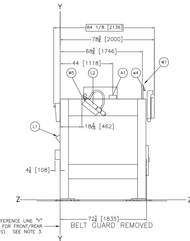
RIGHT VIEW
