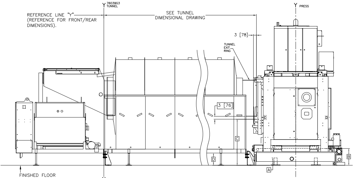
76028 PF TUNNEL/MP1540 SINGLE STAGE PRESS
