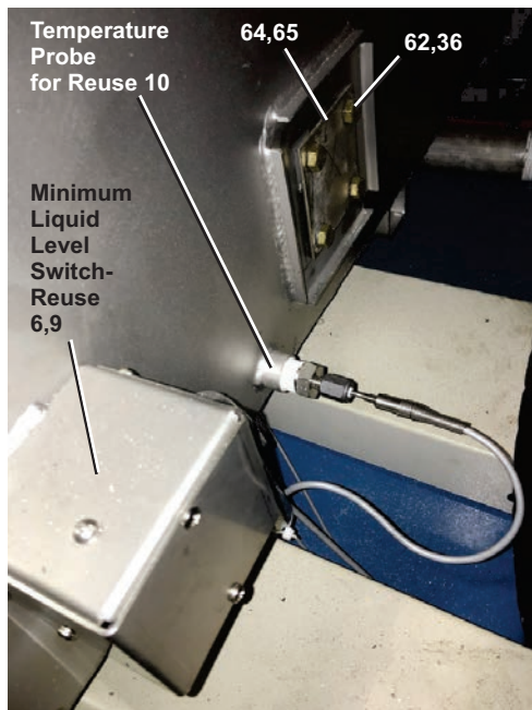
View B-B
