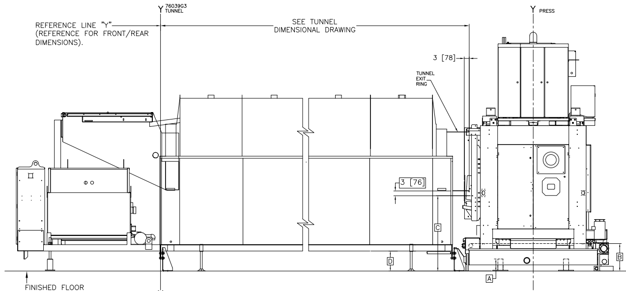
76039 PF TUNNEL/MP1540 SINGLE STAGE PRESS
