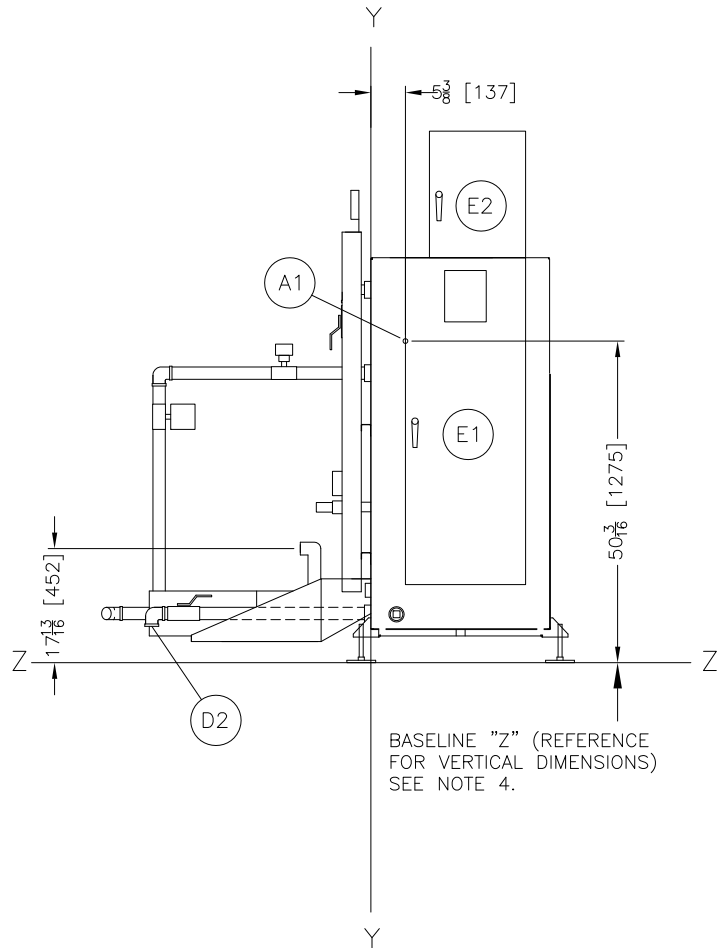
RIGHT VIEW
