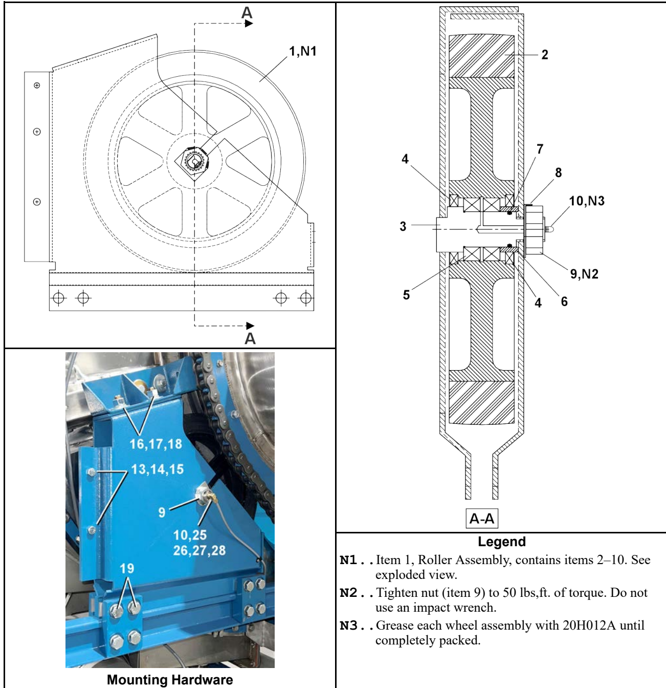
Figure 2. Roller Installation
