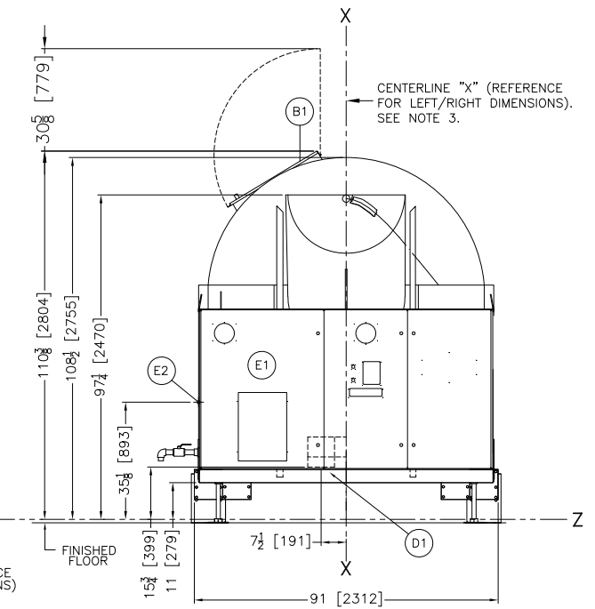
FRONT VIEW LOAD END
