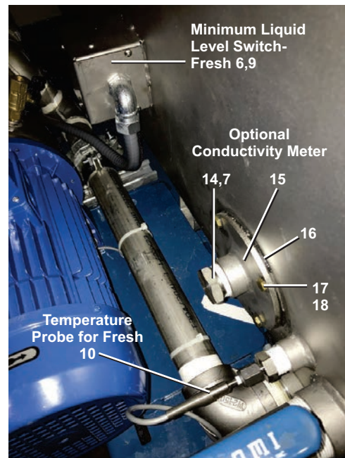
View C-C
