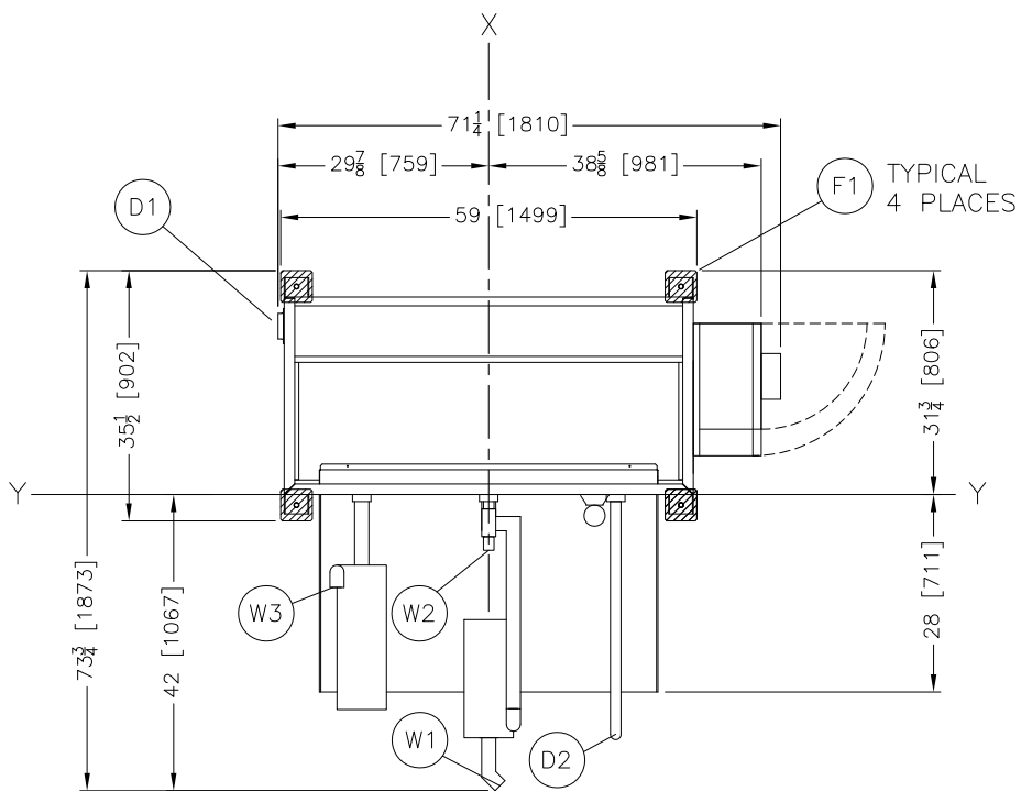
PLAN VIEW
