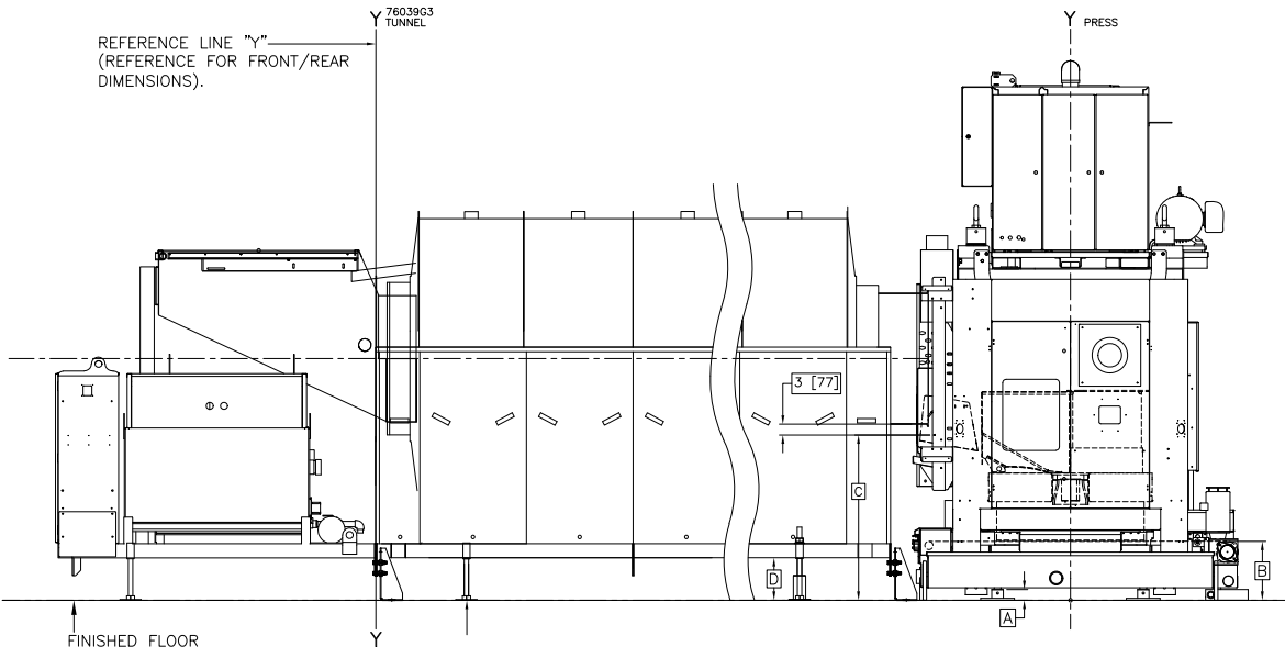
76028 PF TUNNEL/MPL556, MPL640, MPL656 SINGLE STAGE PRESS
