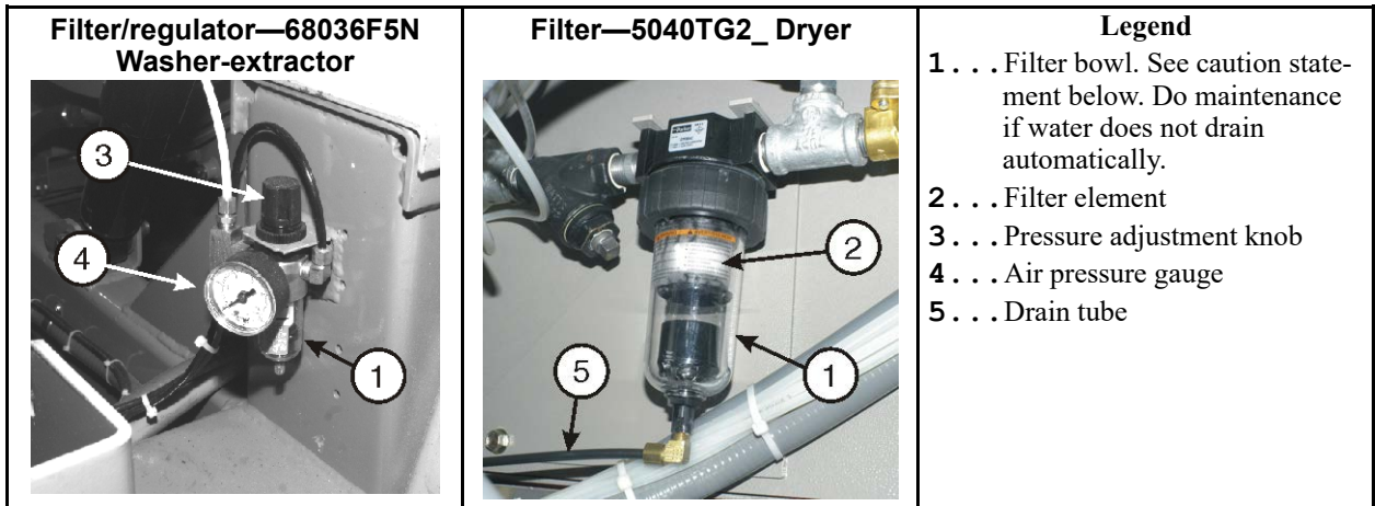
Figure 14. Self-purging Air Line Filter to Remove Moisture and Other Contamination. These are examples. Your machine can look different.
