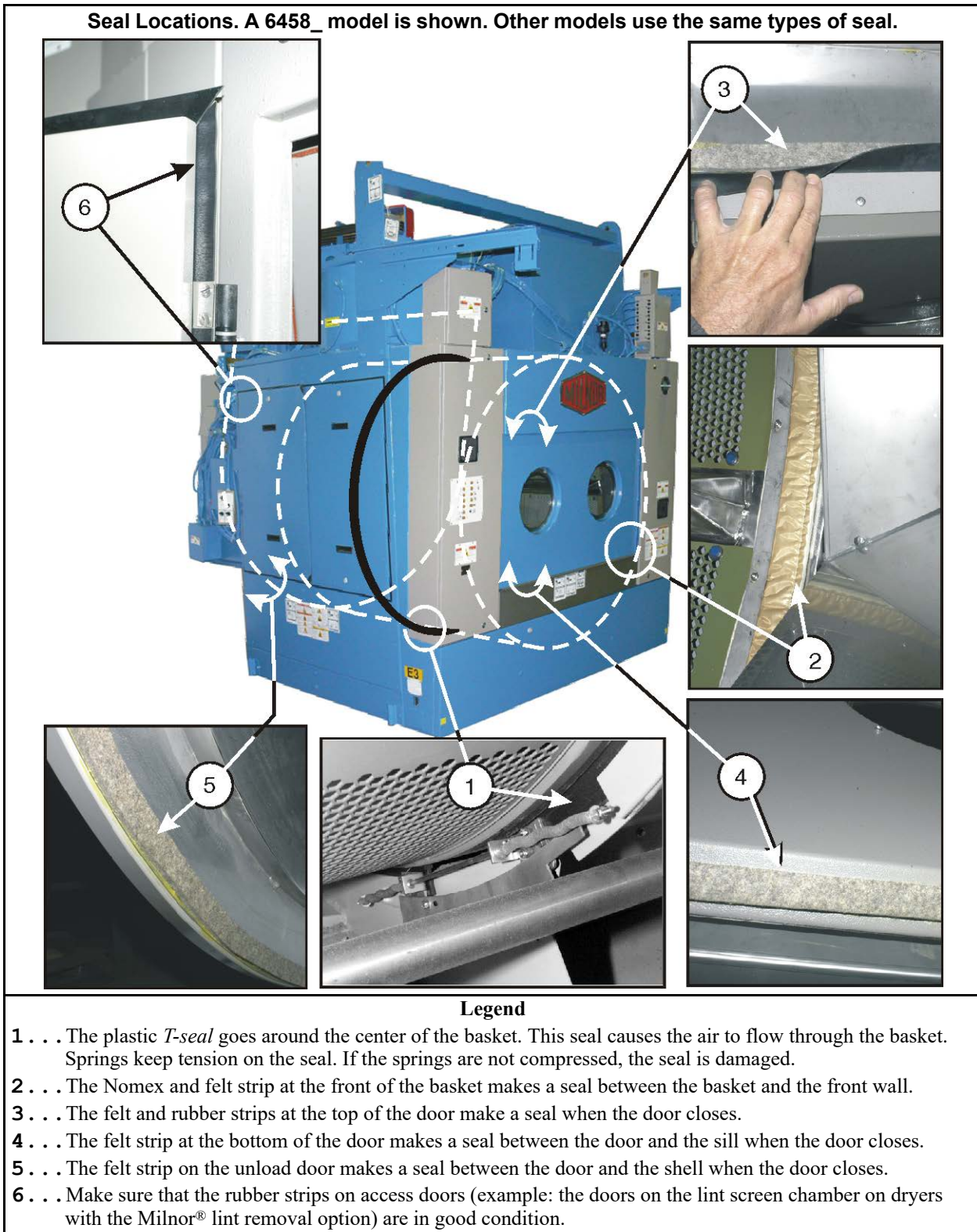
Figure 24. Dryer Air Seals
