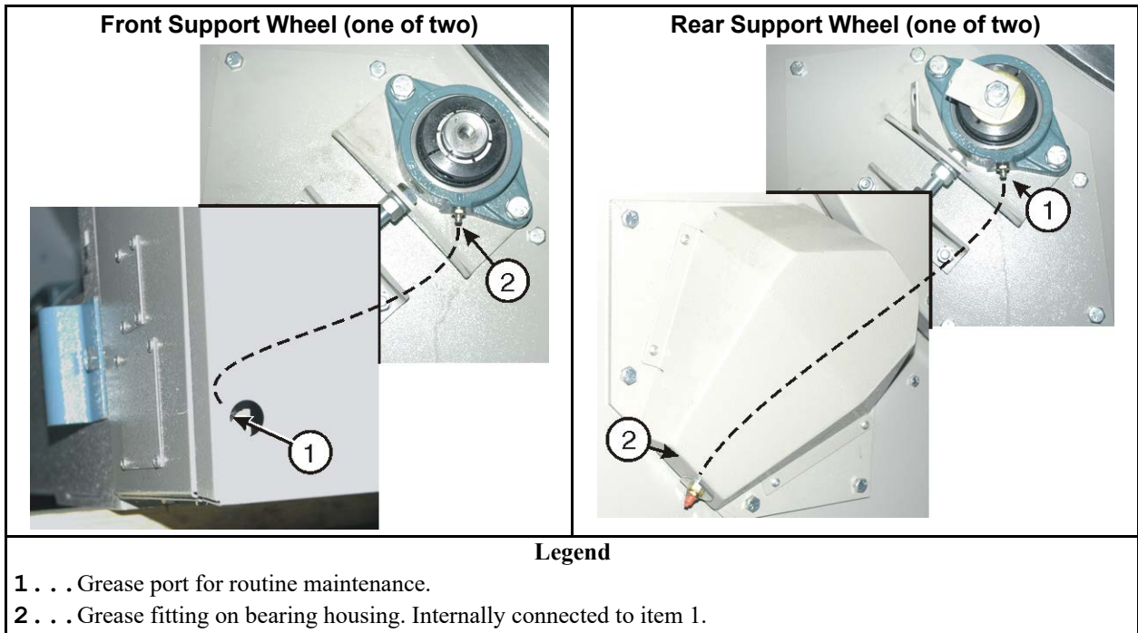
Figure 23. Lubrication of Basket Drive Components
