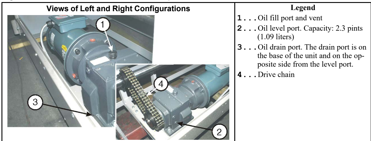
Figure 23. Lubrication of Basket Drive Components
