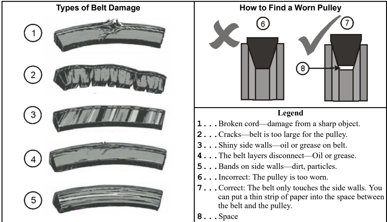
Figure 8. Belt and Pulley Conditions To Look For
