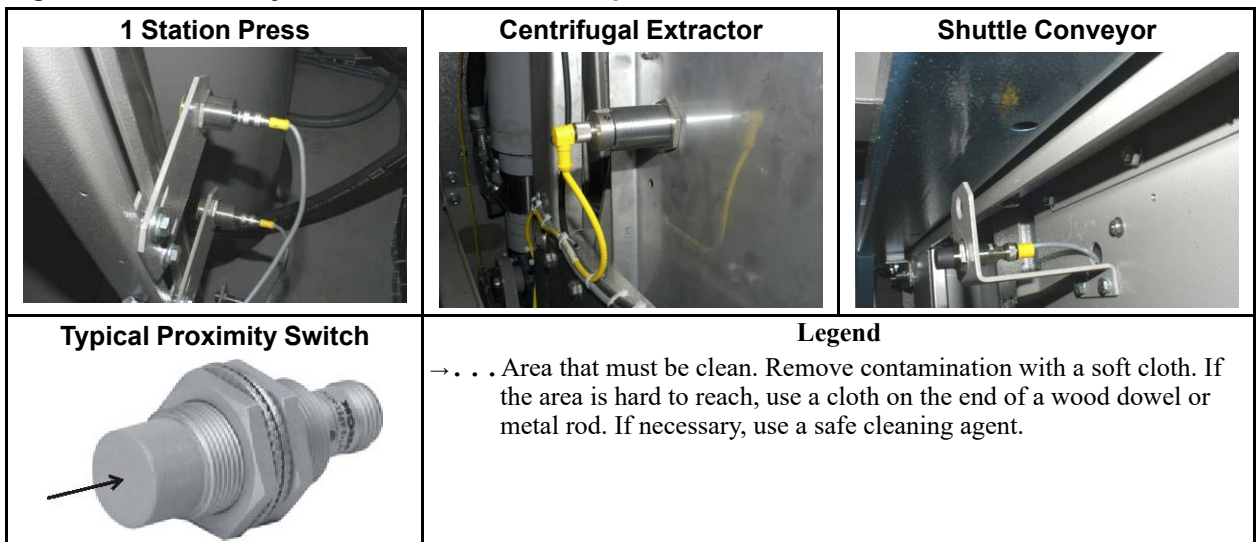
Figure 17. Proximity Switches These are examples. Your machine can look different.
