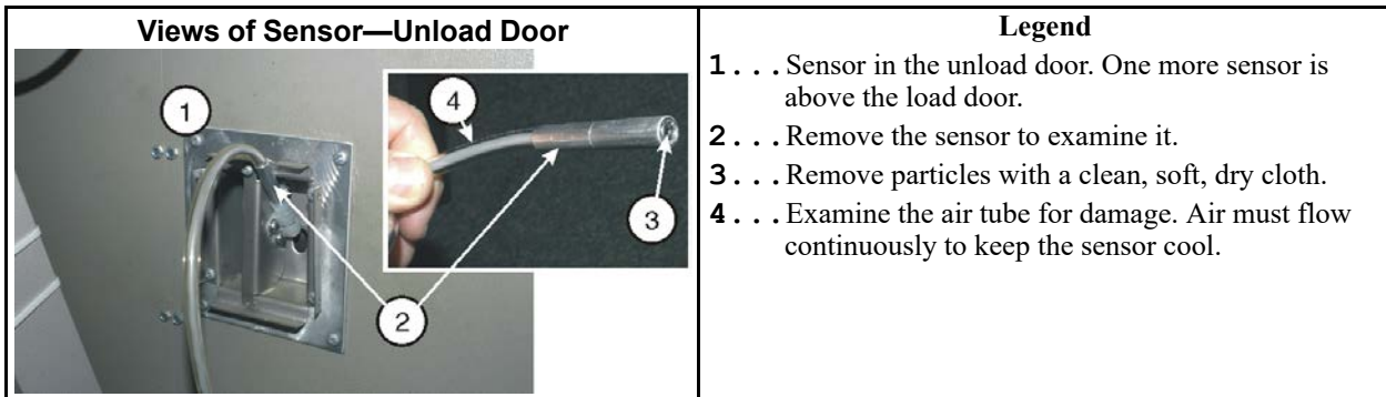
Figure 21. Examine the Sensors—Option for Infrared Temperature Sensing
