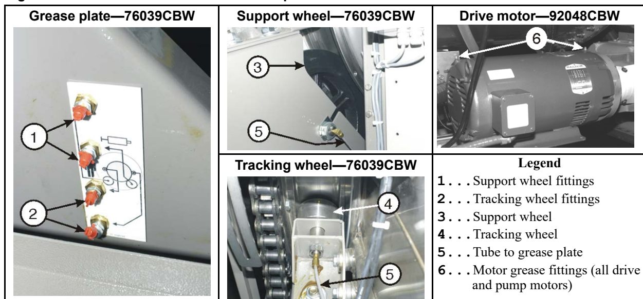
Figure 23. Grease Points. These are examples. Your machine can look different.
