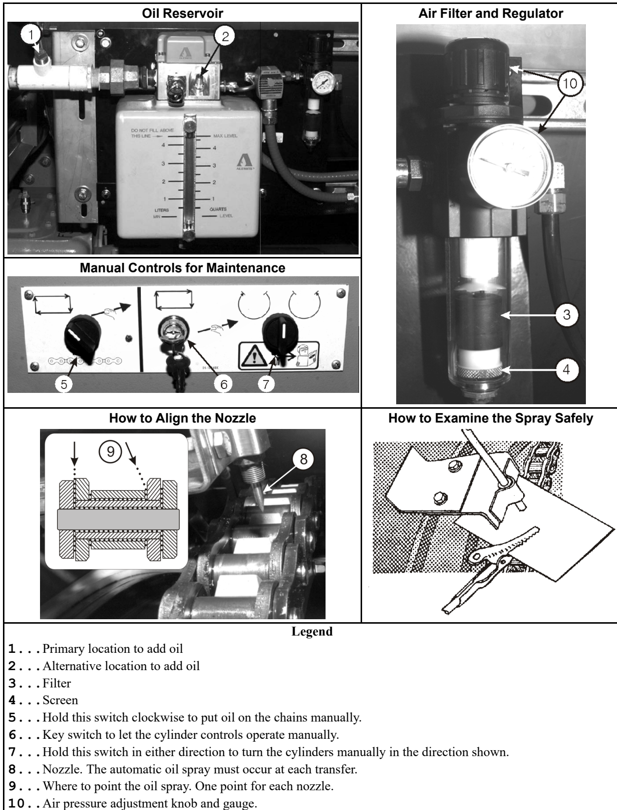
Figure 25. Oil Mist System for Drive Chain
