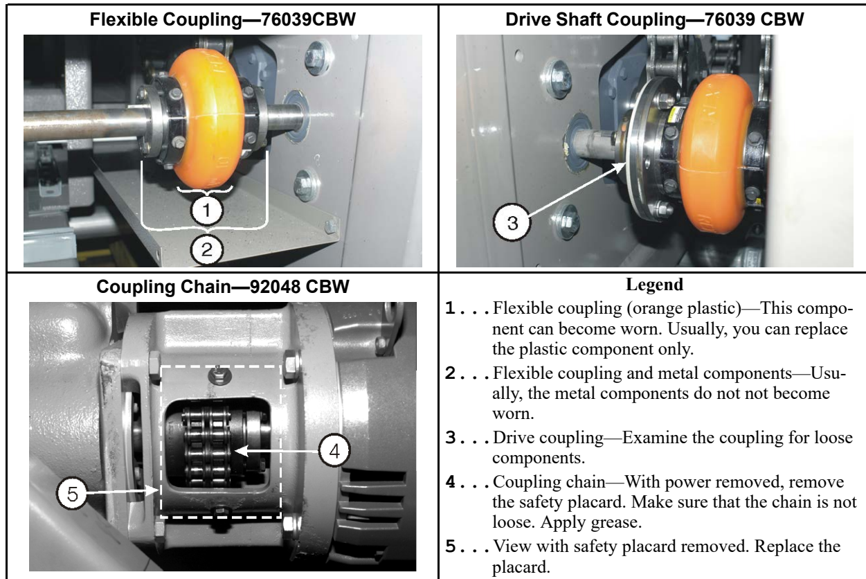
Figure 23. Grease Points. These are examples. Your machine can look different.
