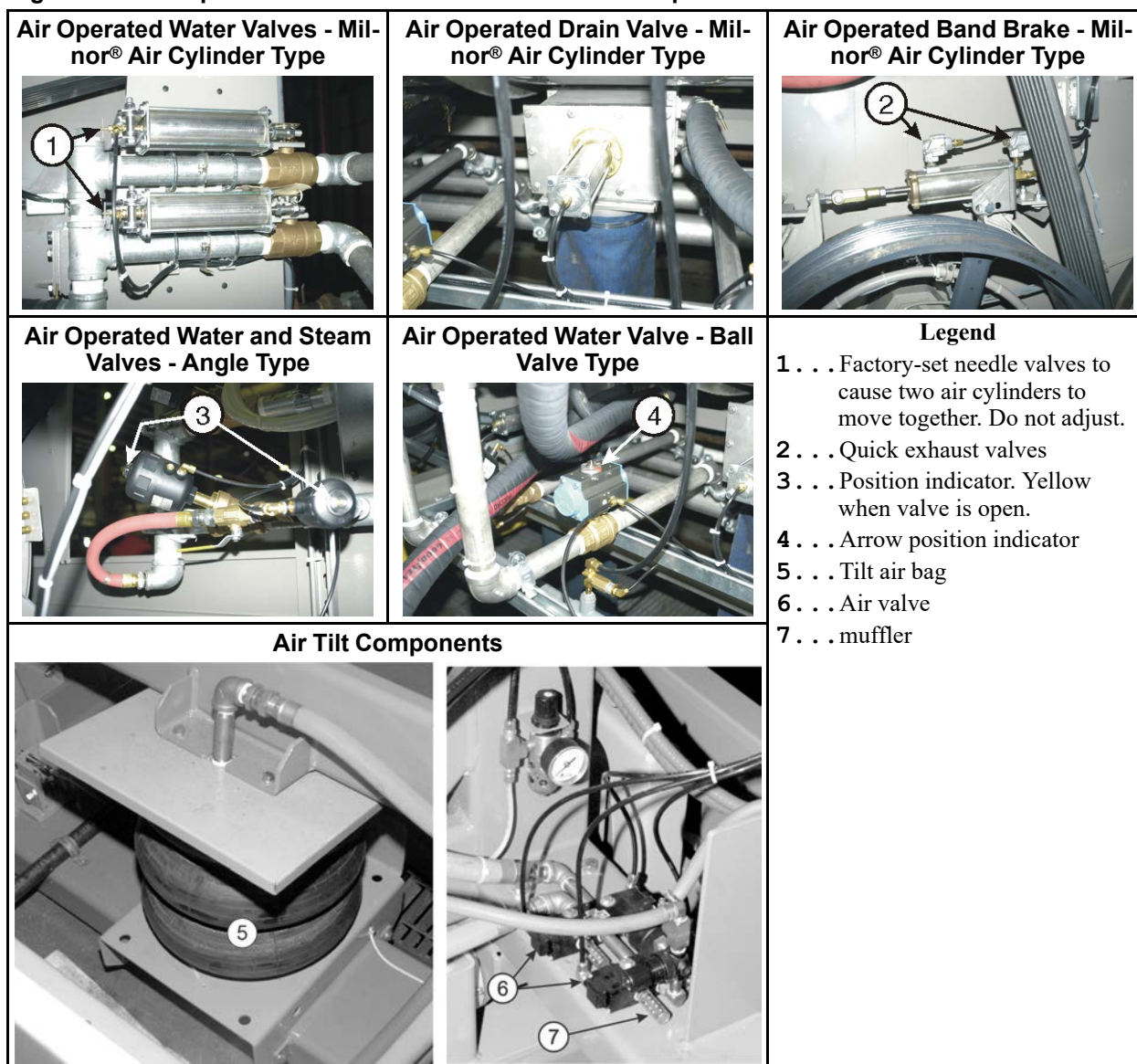
Figure 19. Compressed Air Mechanisms These are examples. Your machine can look different.
