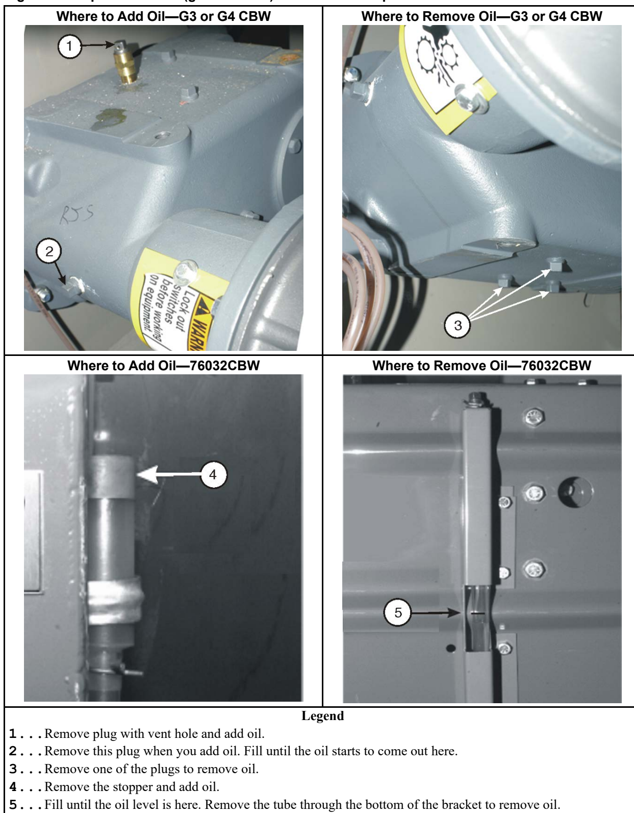
Figure 24. Speed Reducer (gear reducer). These are examples. Your machine can look different.
