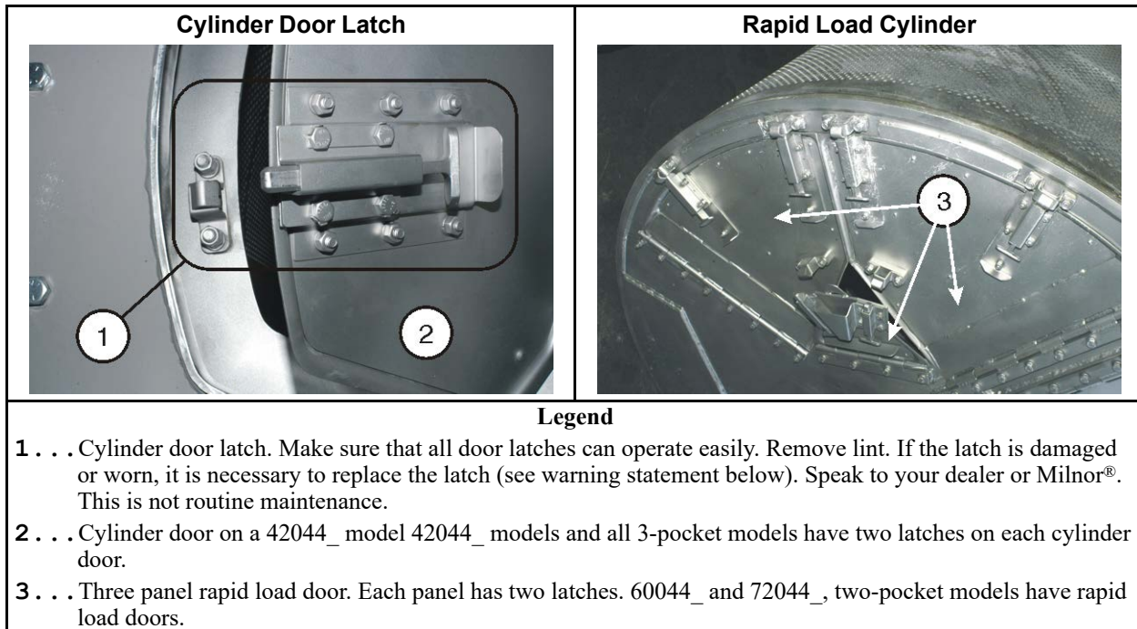
Figure 21. Cylinder Door Latches
