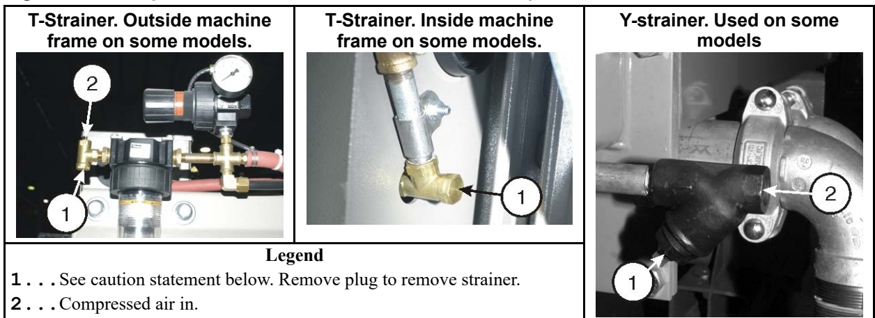
Figure 15. Compressed Air Inlet Strainers. These are examples. Your machine can look different.
