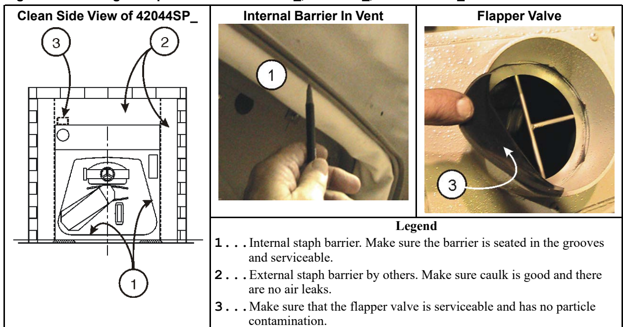
Figure 23. Air Tight Staph Barriers—42044SP_, 60044SP_, and 72044SP_ Models
