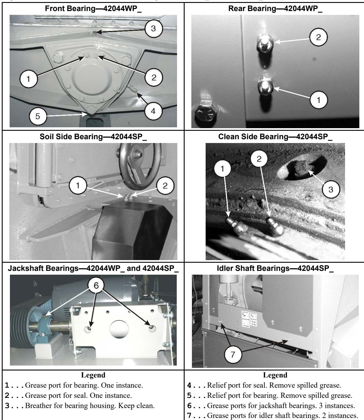
Figure 19. Grease Ports for Drive Bearings—42044WP_ and 42044SP_ Models
