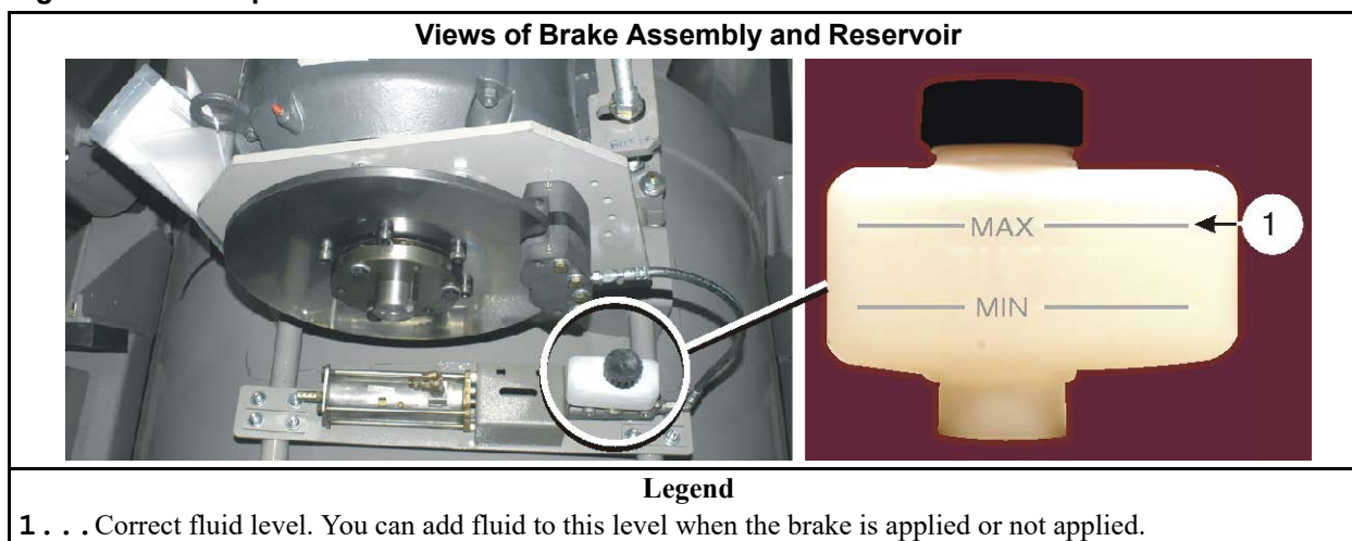
Figure 24. Example of Disk Brake. Your machine can look different.
