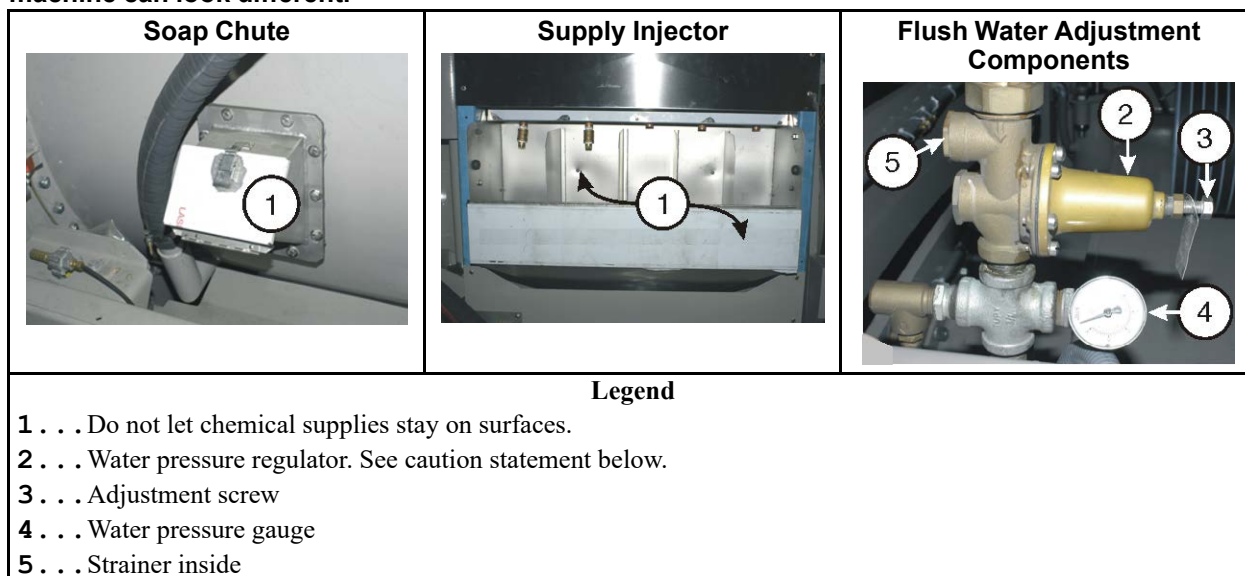
Figure 11. Soap Chute and Optional 5-compartment Supply Injector. These are examples. Your machine can look different.
