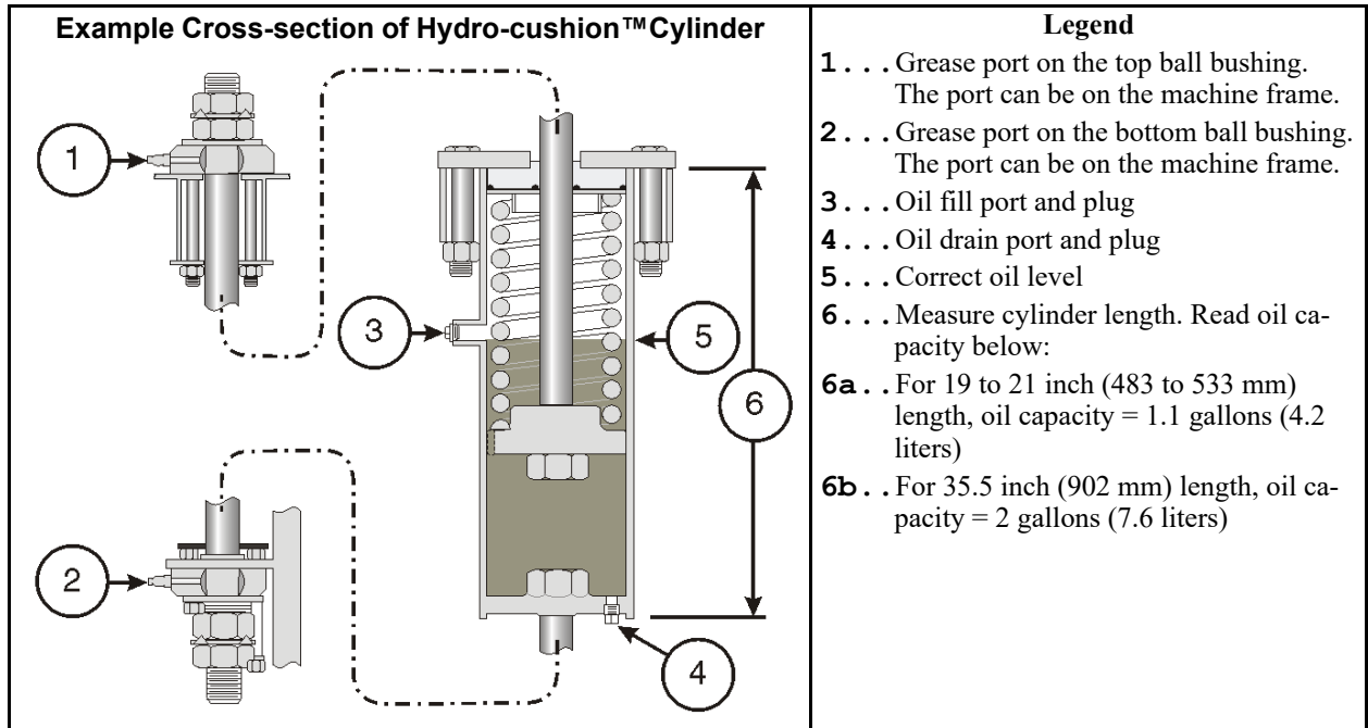
Figure 22. Grease Ports, Oil Ports, and Approximate Oil Capacity for Hydro-cushion™ Cylinders
