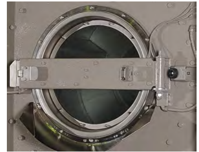
Figure 5. Air-unlatch Door
