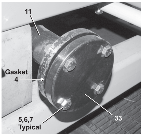
Steam Manifold - Last Module
