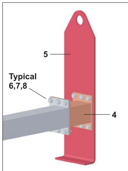
Detail B:
