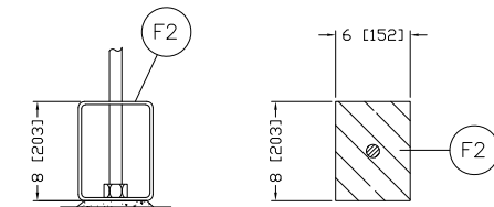
ADJUSTABLE FOOT
