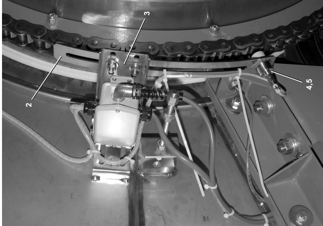
Clockwise Limit Switch (A)
