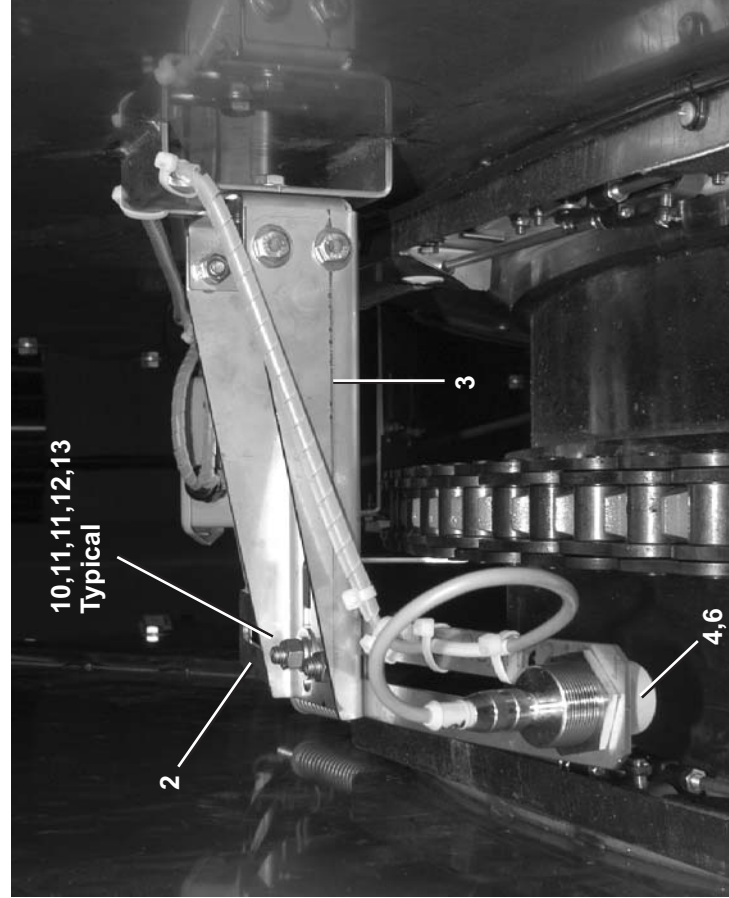
Top-Dead-Center Limit Switch (C)
