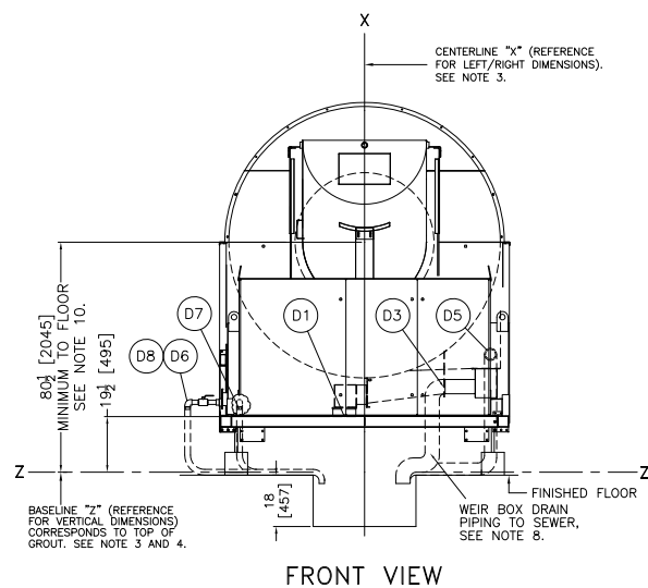
FRONT VIEW CENTER DRAIN TROUGH (SEE NOTES 7 & 8. SEE FIGURE 1.)
