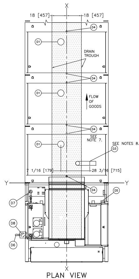
PLAN VIEW
