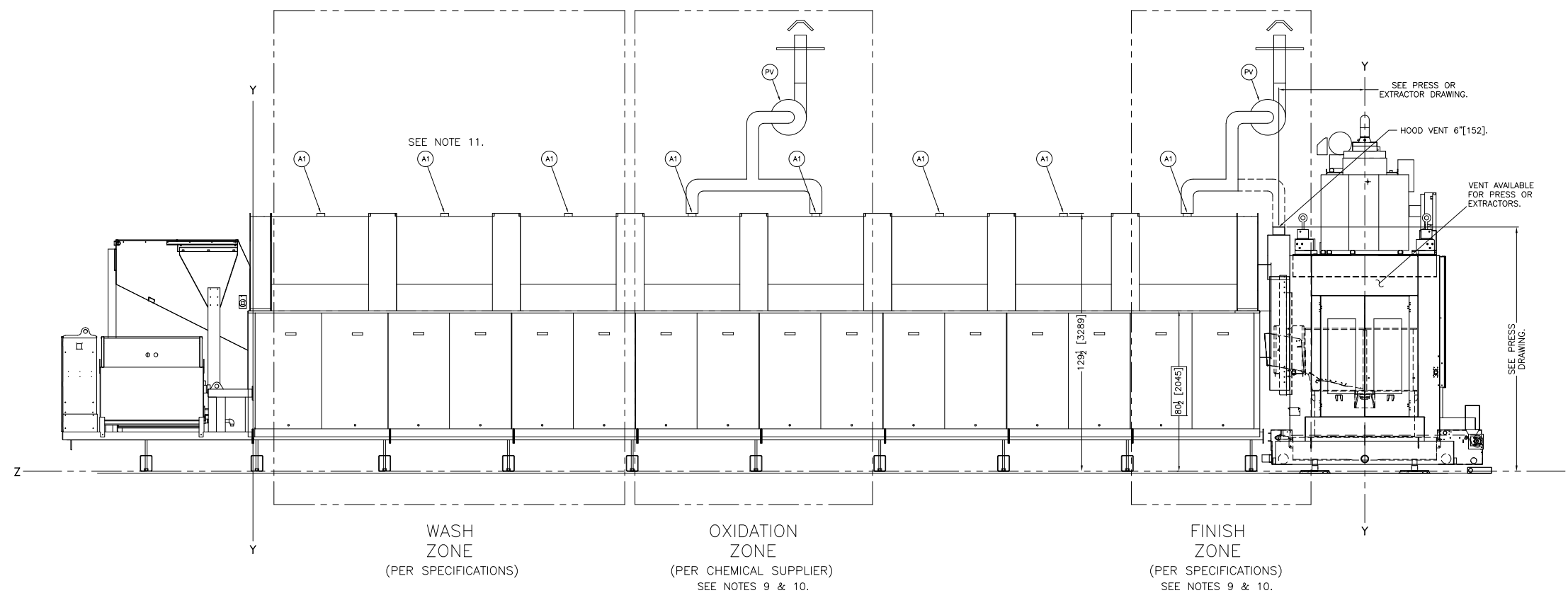
RECOMMENDED VENT SYSTEM FOR THE 9248G4 TUNNEL WASHER AND ADJACENT PRESS
