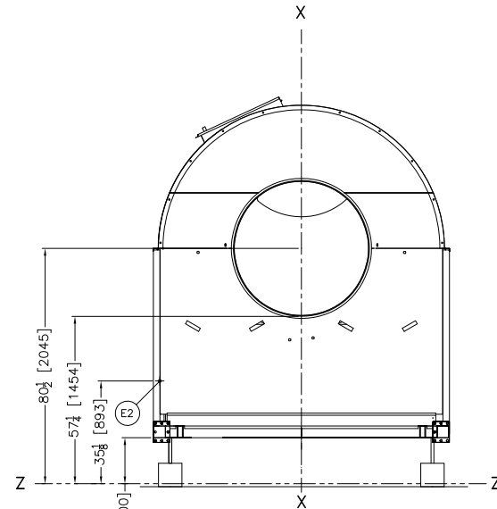
REAR VIEW
