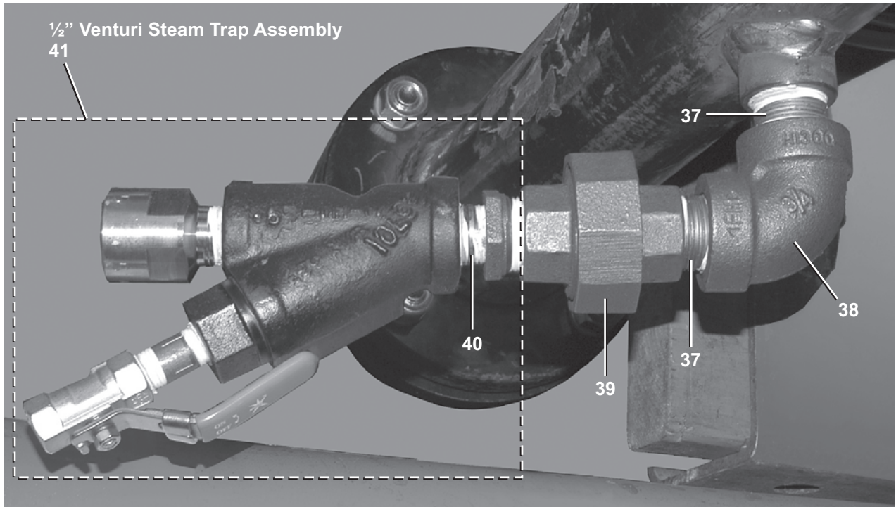
Steam Trap Installation - Last Module
