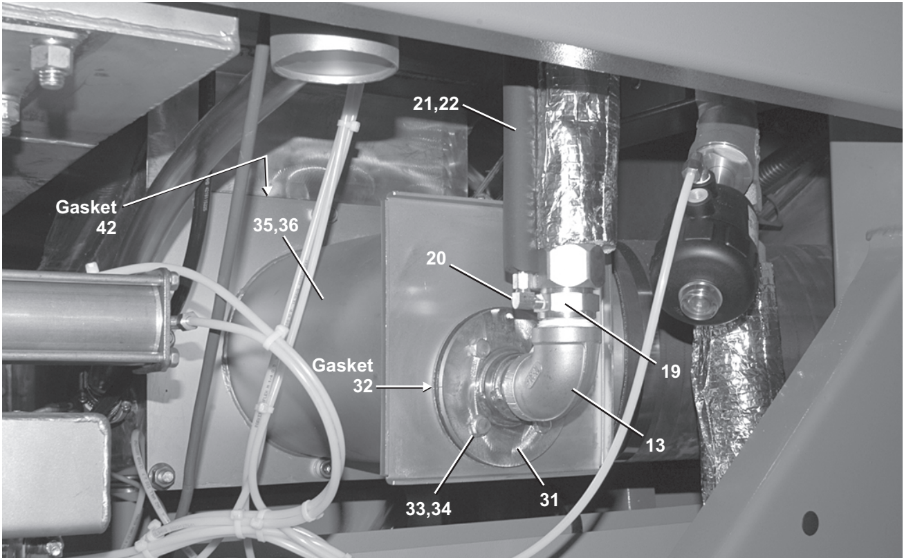
Steam Sparger Tube
