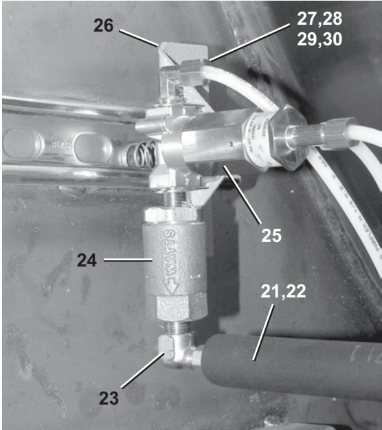
Asperator Assembly
