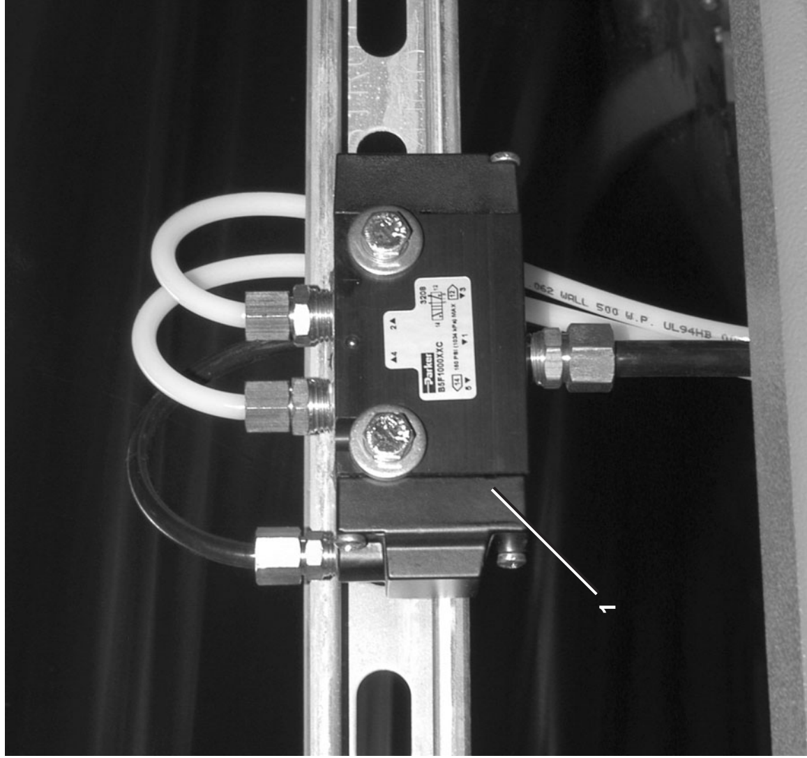
5 Port, 4 Way, 2 Position, Spring Return Valve
