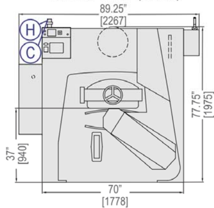
FOUNDATION VIEW
