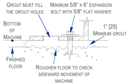
ANCHORING DETAIL
