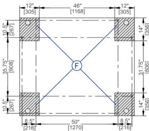
FOUNDATION VIEW
