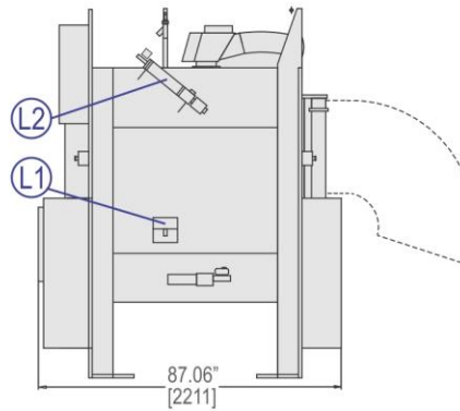
ANCHORING DETAIL
