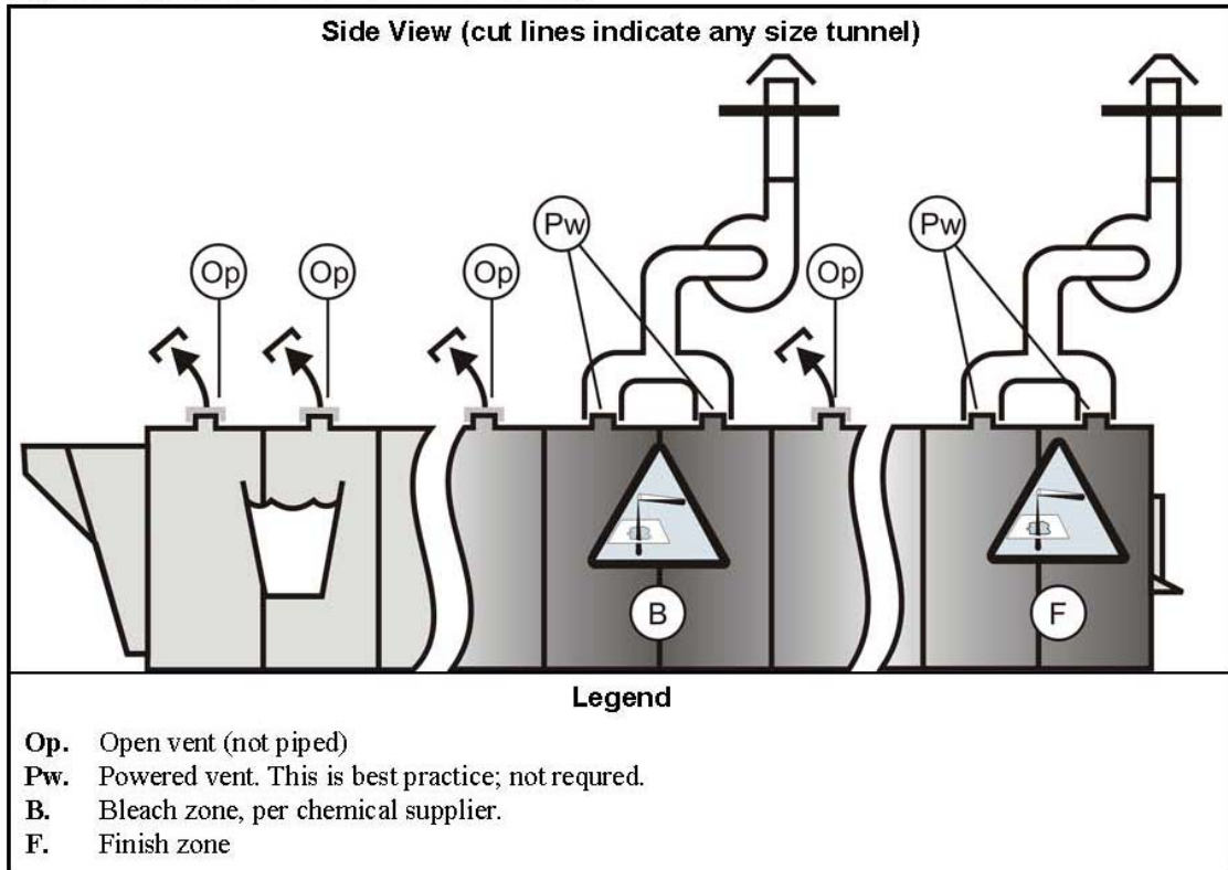
Figure 1: Typical CBW® Tunnel Washer Venting
