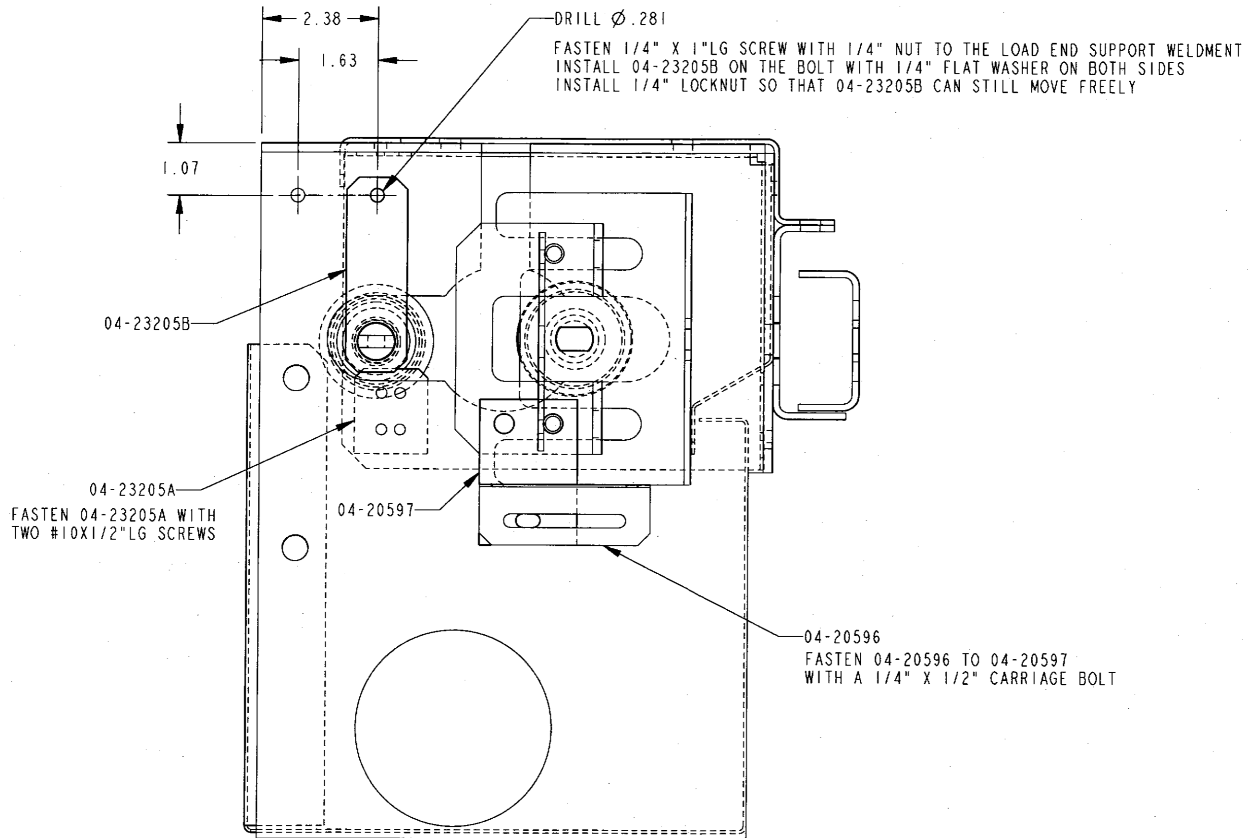
SSPRESS SNUBBER PIVOT BRACKET INSTALLATION
